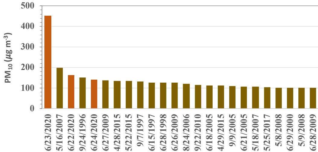
(b) 24 extreme events since 1994 ( \text{PM}_{10} > 100 \mu\text{g m}^{-3} )
