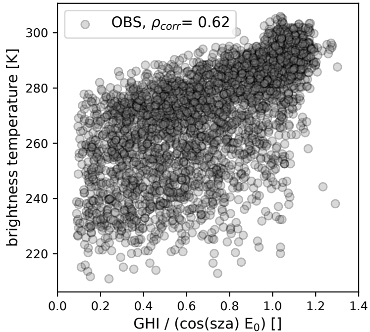
(b) IR108
