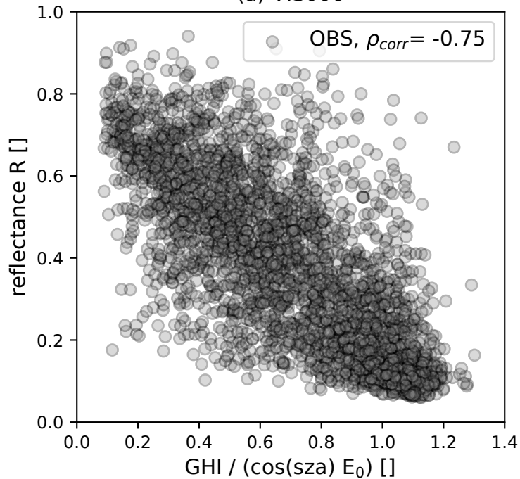
(a) VIS006
