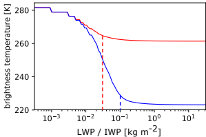
(b) IR108
