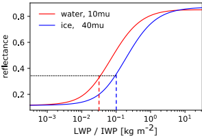
(a) VIS006
