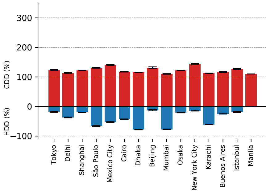
(b) CDD and HDD Change in 2.0 °C
