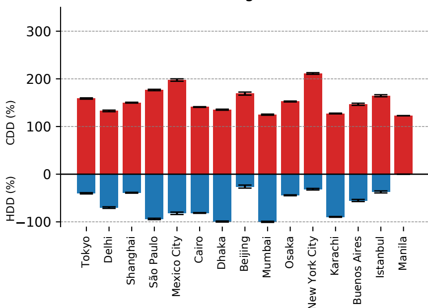
(c) CDD and HDD Change in 3.0 °C
