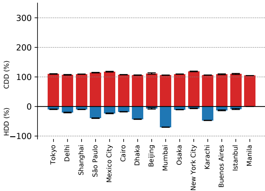
(a) CDD and HDD Change in 1.5 °C
