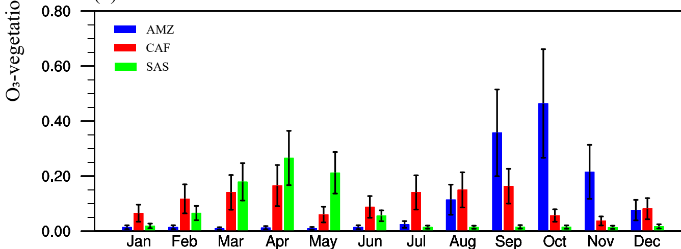
(b) Fire alone emissions
