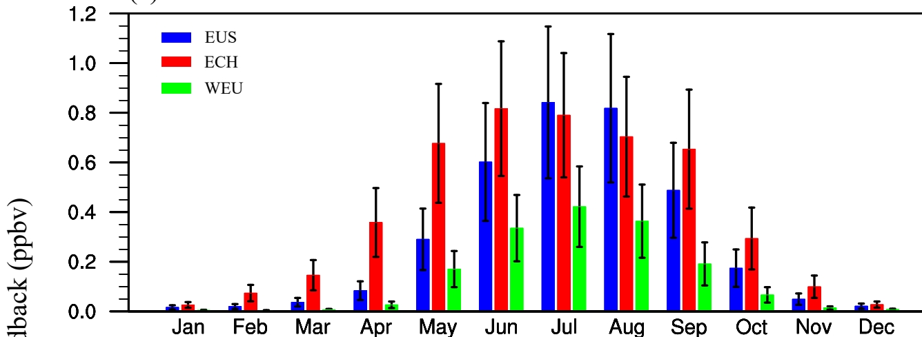
(a) Emissions without fire
