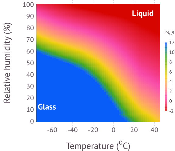
(b) Citric Acid
