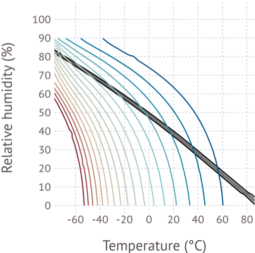
(a) Sucrose
