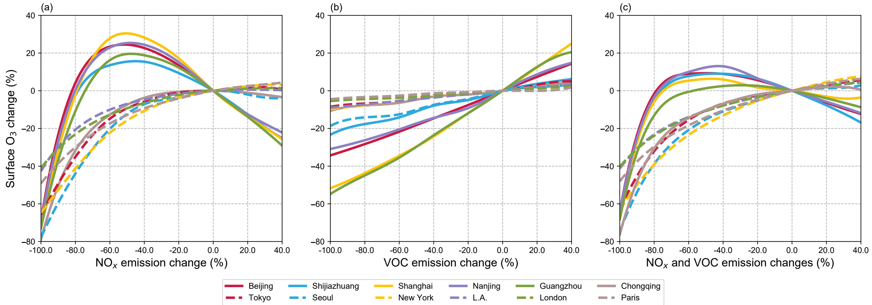
O 3 responses to NO x , VOCs and combined emission changes for the global regions in JJA, 2016
