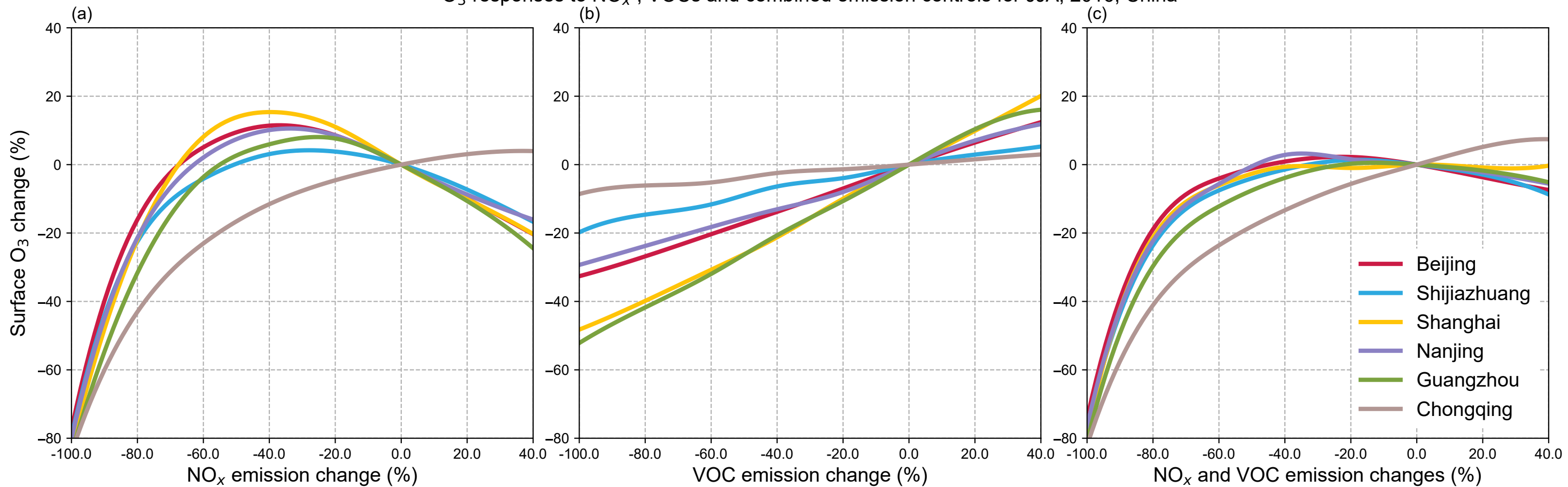
O 3 responses to NO x , VOCs and combined emission controls for JJA, 2016, China
