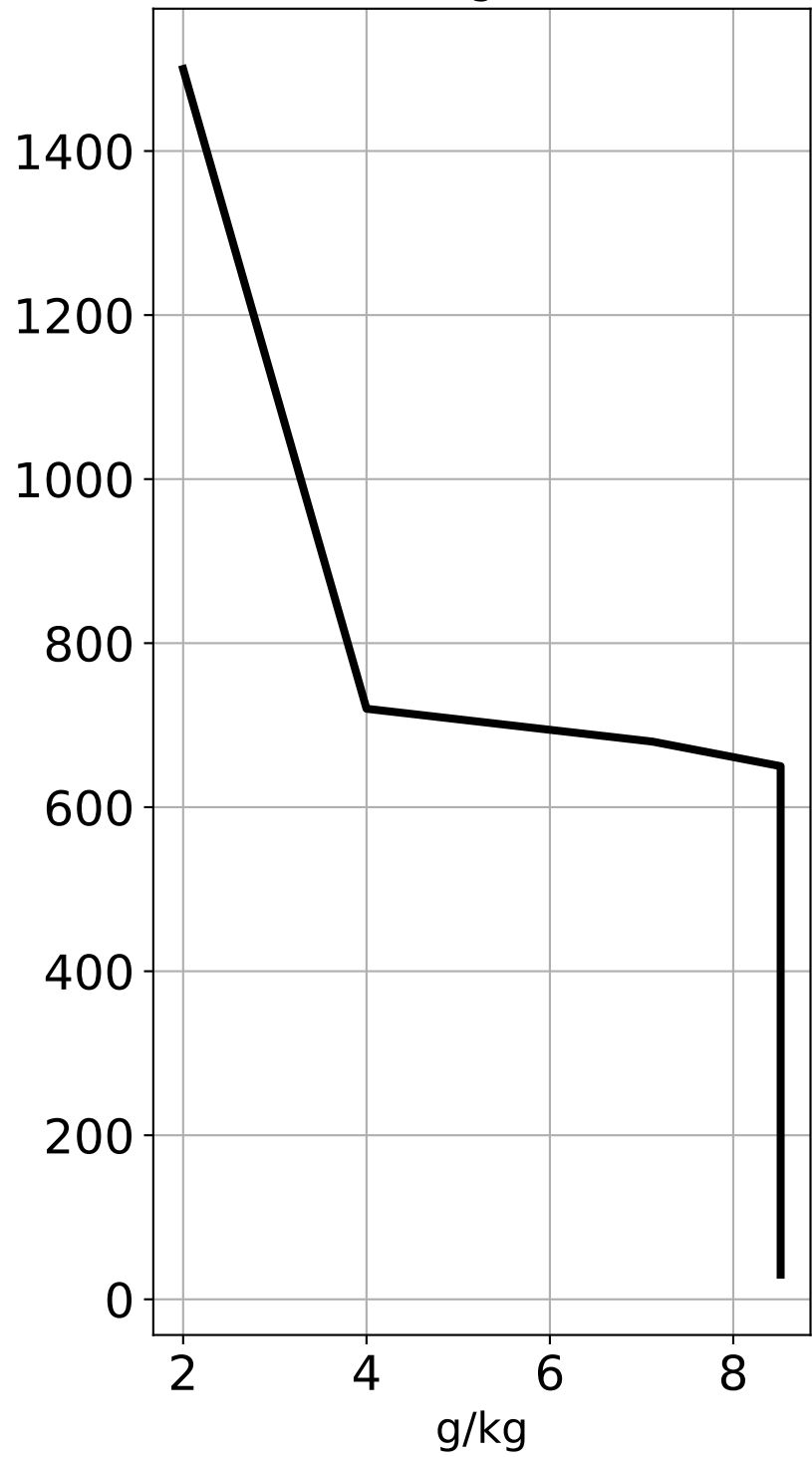
Mixing ratio
