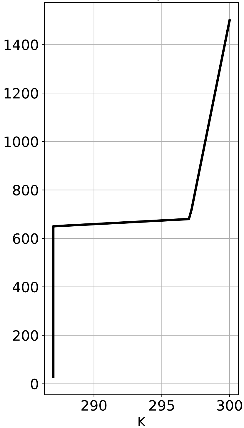
Potential temperature
