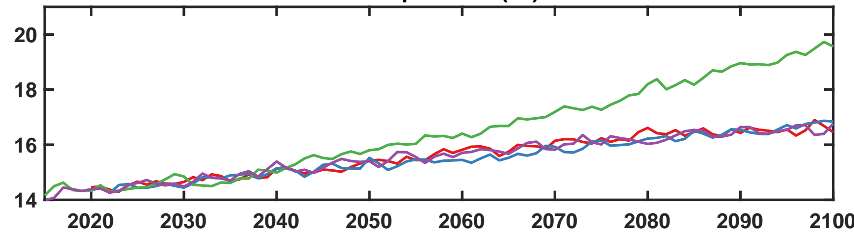
Global Surface Air Temperature (°C) - IPSL-CM6A-LR
