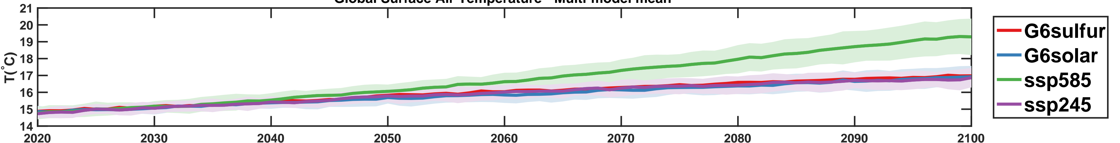
Global Surface Air Temperature - Multi-model mean
