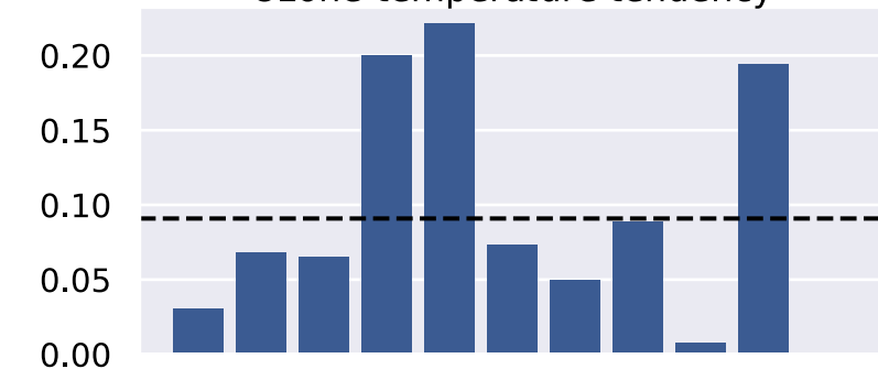
Ozone-temperature tendency
