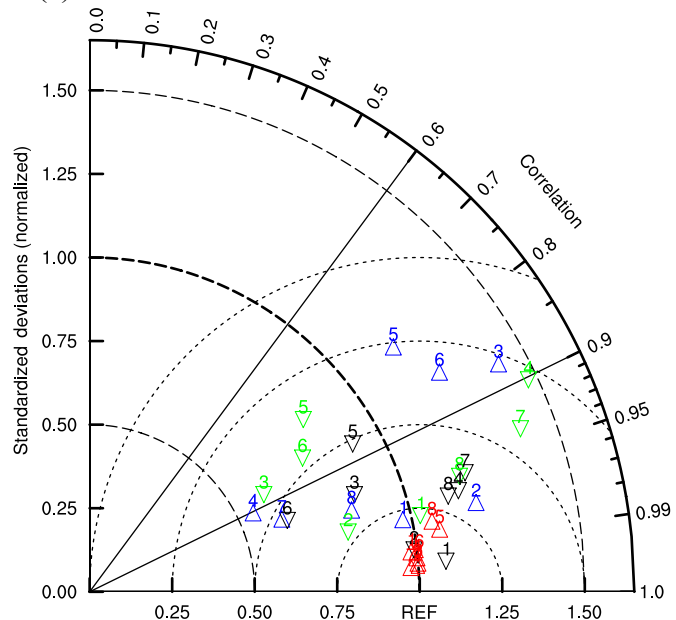
(c) Ventilation coefficient
