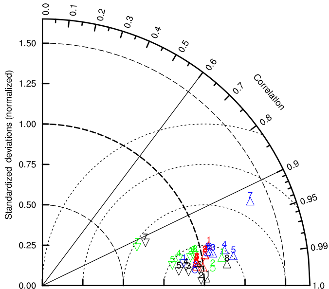
(c) Ventilation coefficient
