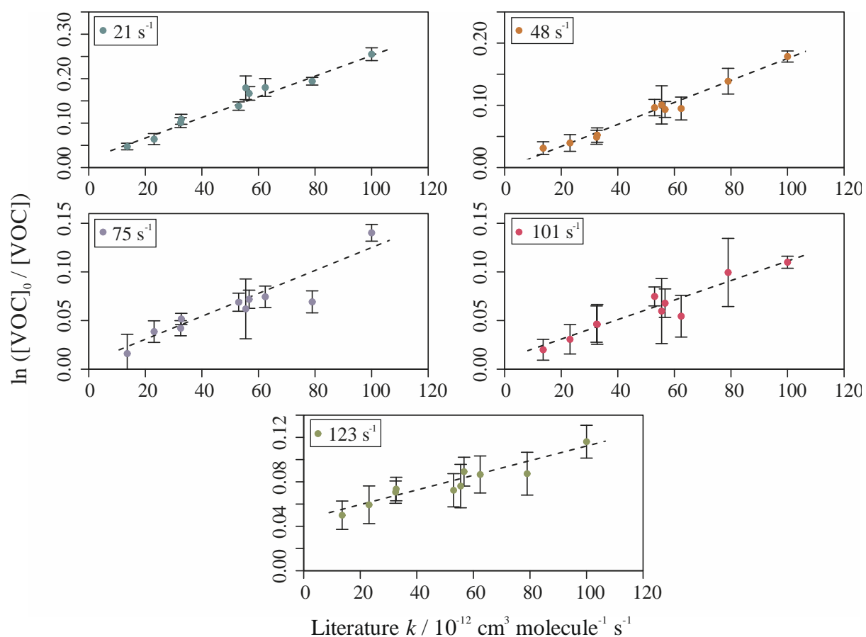
Figure S4. Relative rate plots for Mixture 1 with OH reactivities of 21, 48, 75, 101 and 123 \text{s}^{-1} . The R^2 for the weighted linear fits were 0.958, 0.980, 0.907, 0.967 and 0.829 respectively. The values of OH_{exp} were 2.3 (\pm 0.1) , 1.8 (\pm 0.1) , 1.2 (\pm 0.2) , 1.0 (\pm 0.1) and 0.7 (\pm 0.1) \times 10^9 molecules \text{cm}^{-3} \text{s} respectively.
