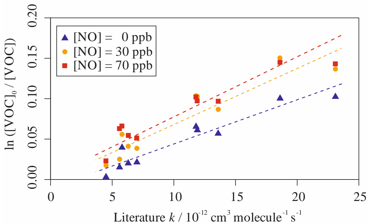
Figure S3. Relative rate plots for Mixture 2 (OH reactivity of 18 \text{ s}^{-1} ) with NO concentrations of 0, 30 and 70 ppbv at 296 (\pm 2) \text{ K} . The calculated OH_{exp} was equal to 5.5 (\pm 0.6) , 6.9 (\pm 0.9) and 7.5 (\pm 0.8) \times 10^9 \text{ molecules cm}^{-3} \text{ s} respectively. The R^2 values for the weighted linear fits were 0.899, 0.853 and 0.909 for [NO] = 0, 30 and 70 ppbv respectively.
