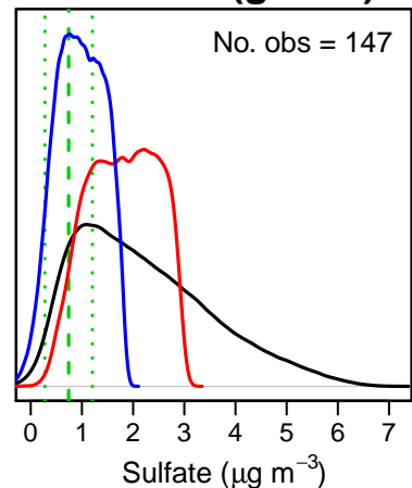
Sulfate (global)
