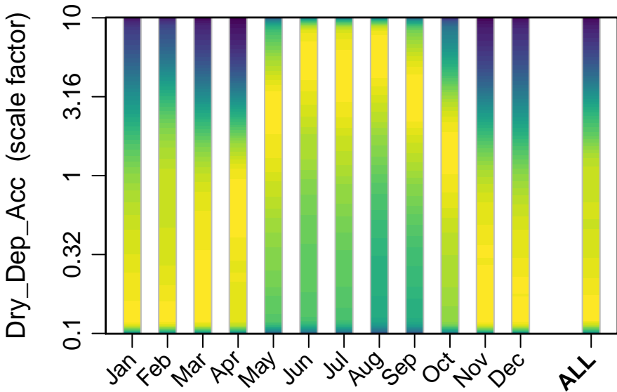
(c) Dry_Dep_Acc constrained by PM 2.5
