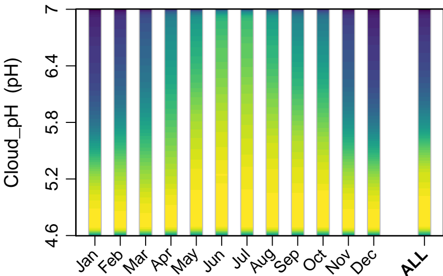
(a) Cloud_pH constrained by AOD
