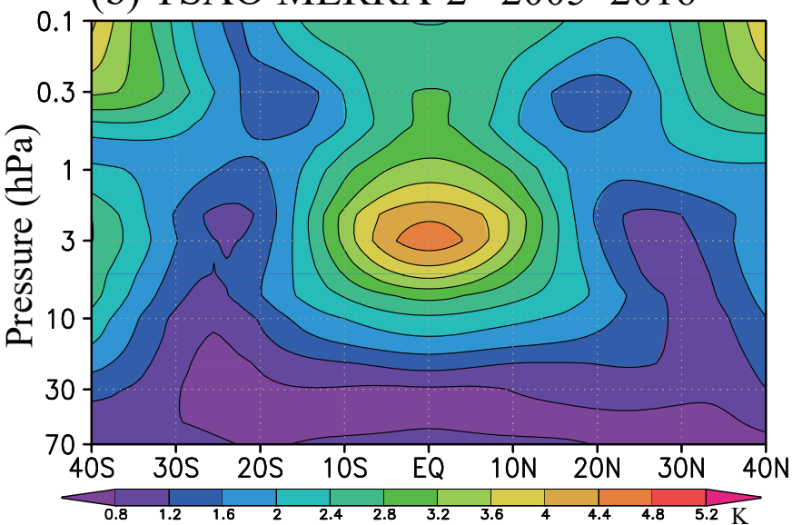
(c) TSAO over the equator
