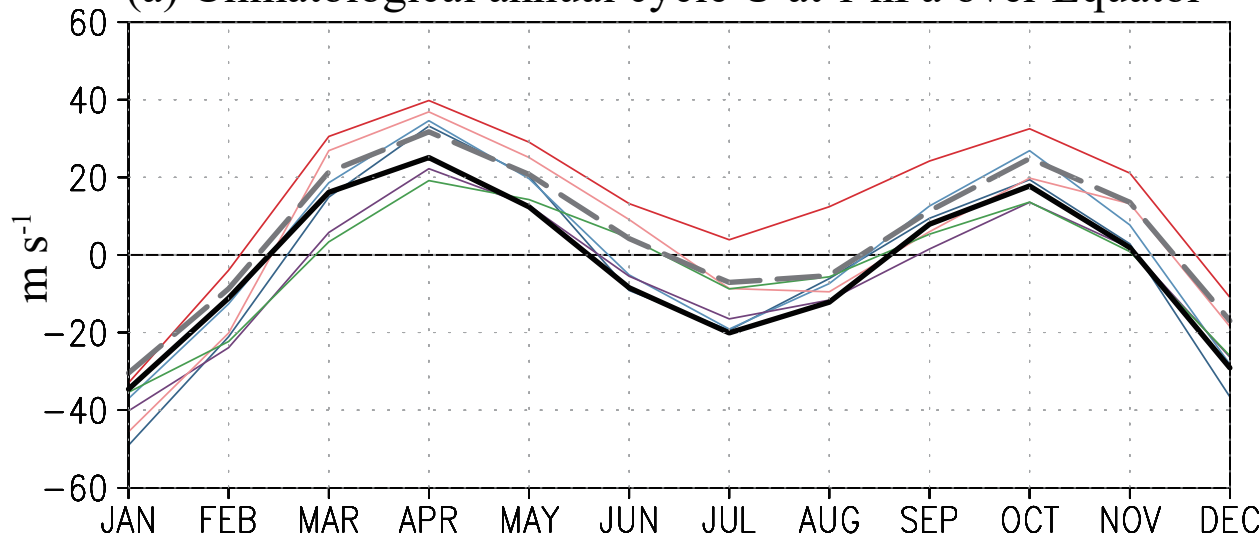
(b) Cycle-to-cycle variability U at 1 hPa over Equator
