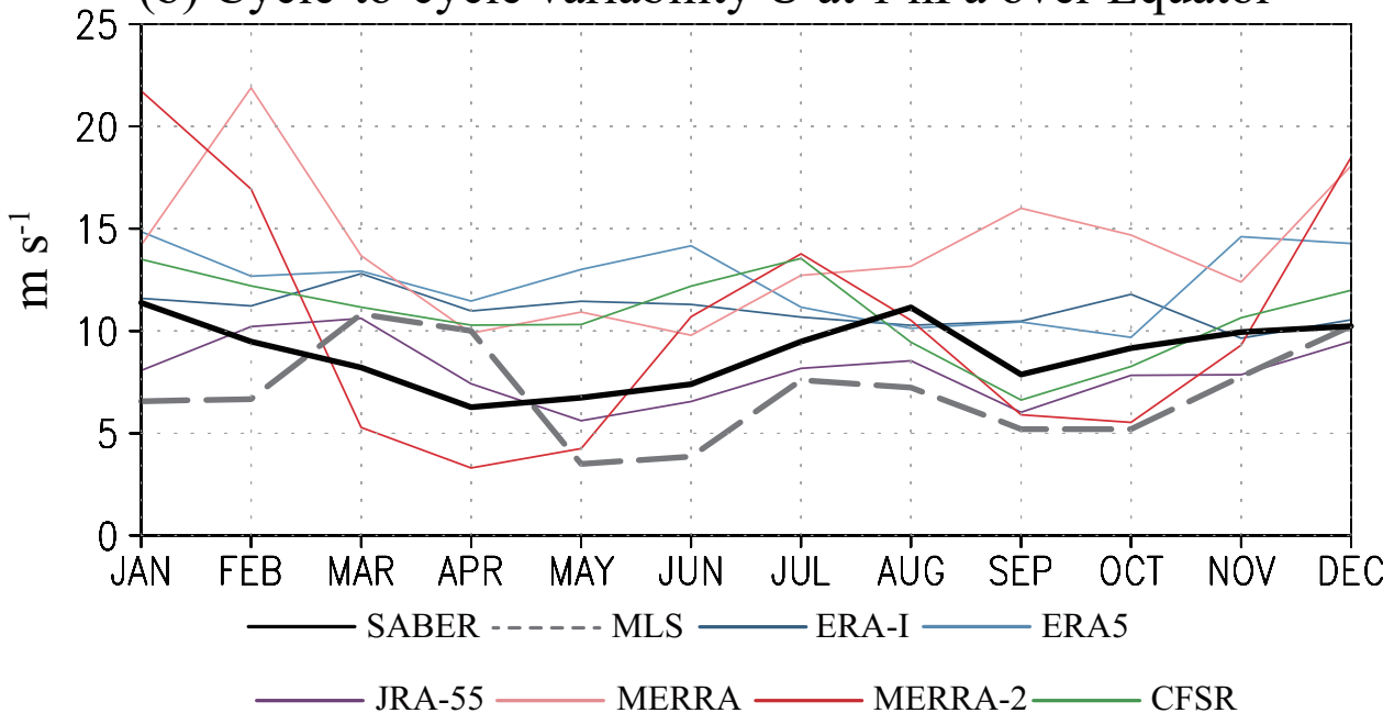
(b) Cycle-to-cycle variability U at 1 hPa over Equator
