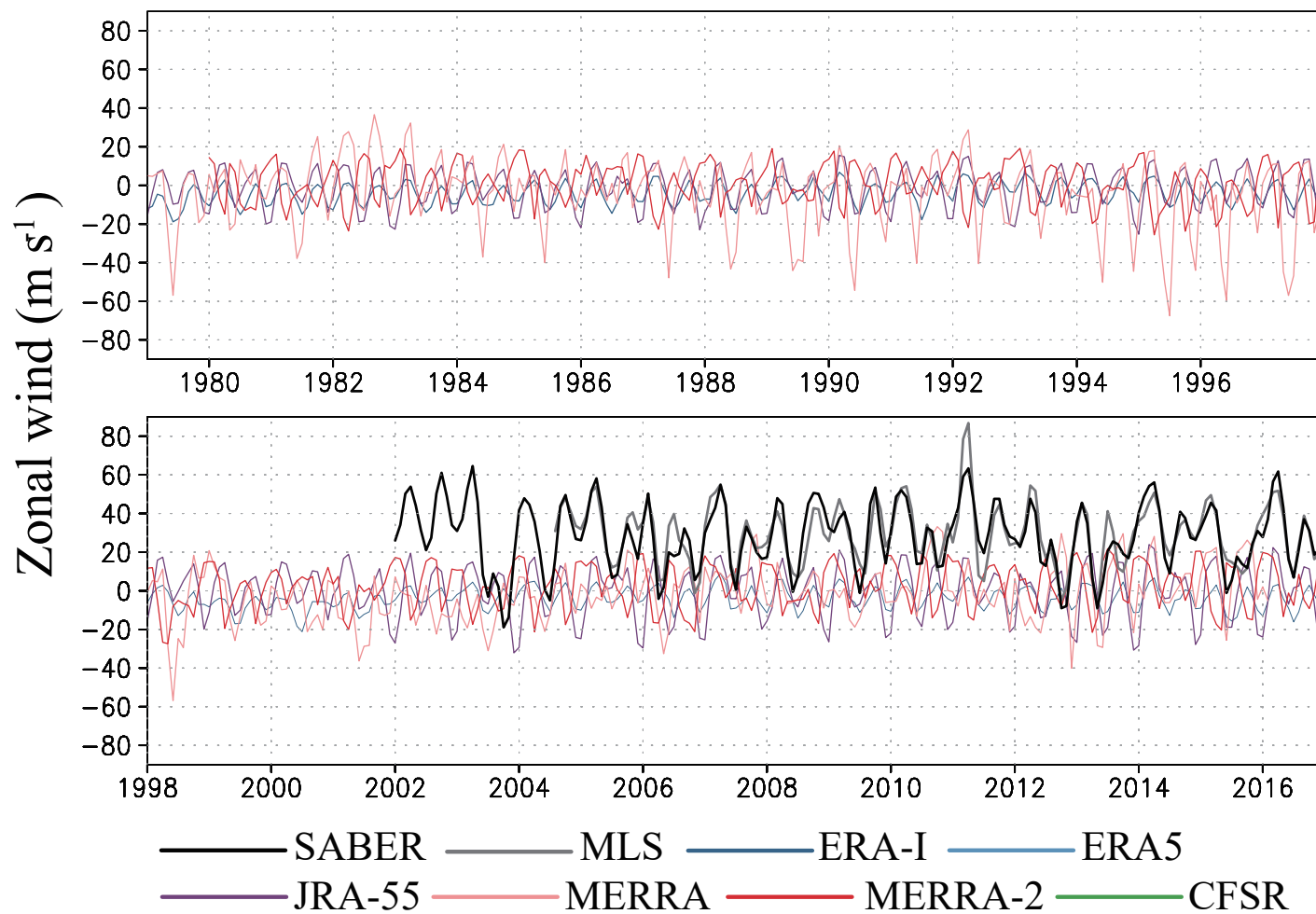
(b) Equatorial zonal mean zonal wind at 0.1 hPa
