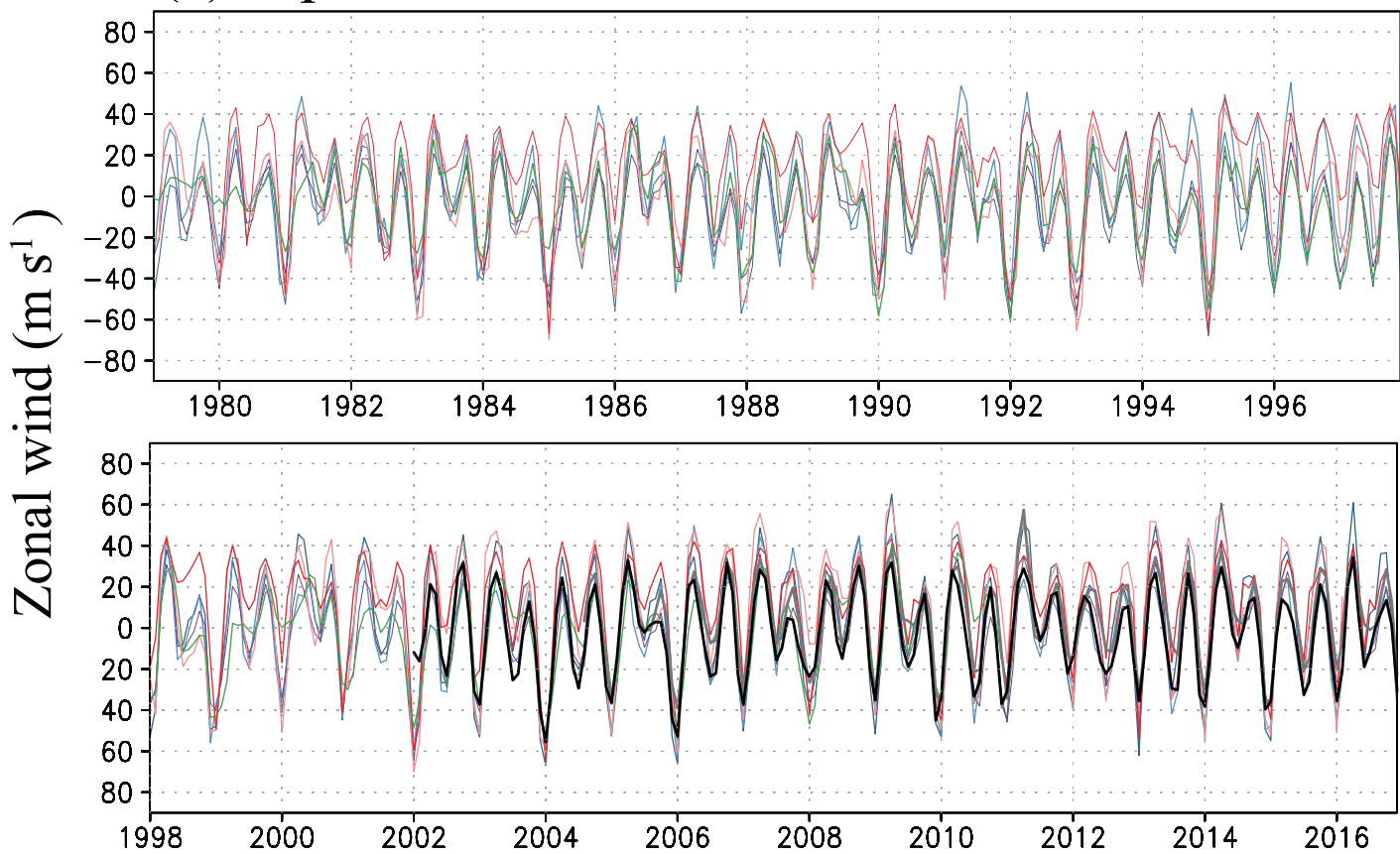
(a) Equatorial zonal mean zonal wind at 1 hPa
