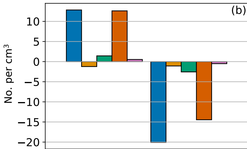
Close to source: difference
