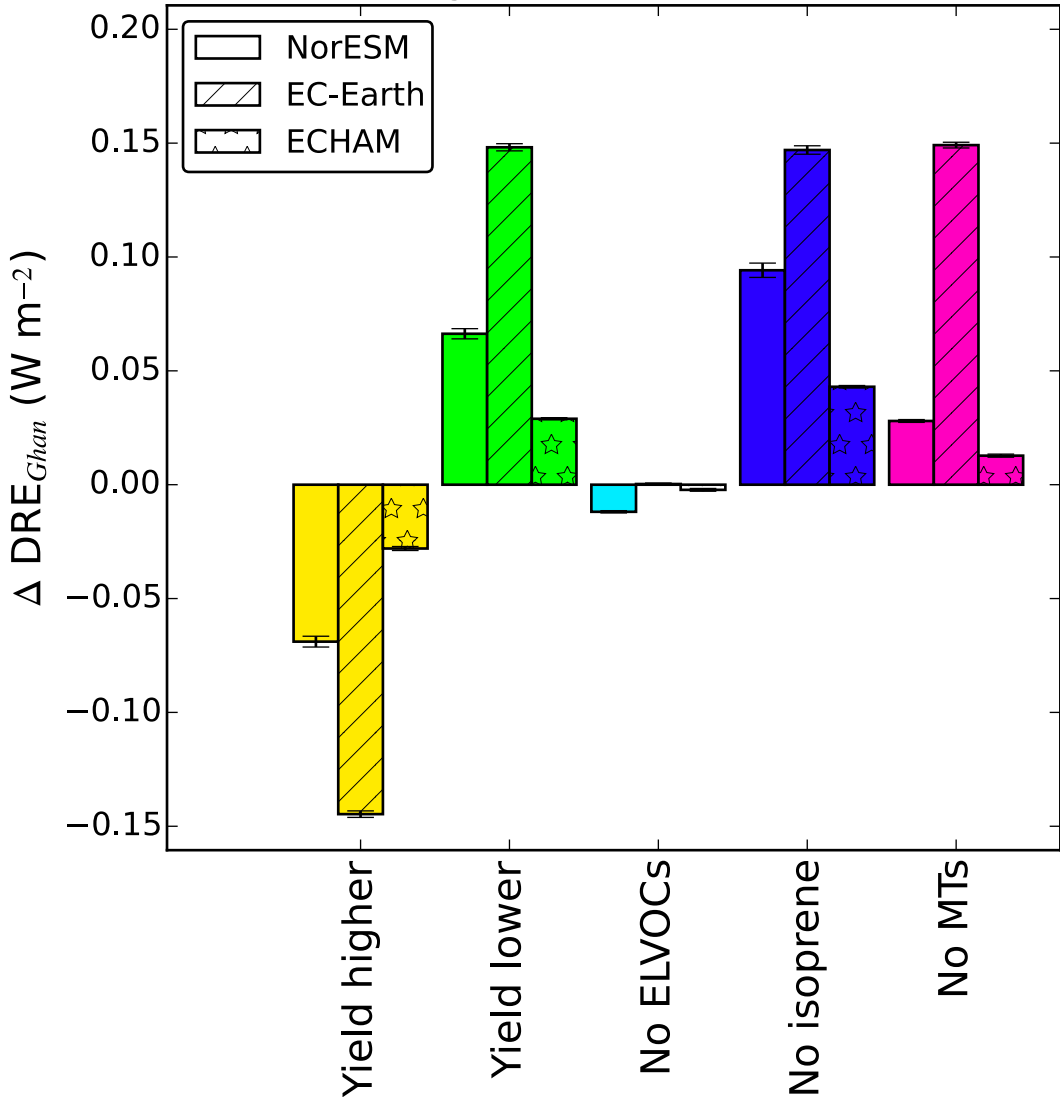
Global average, abs. difference w.r.t. CTRL
