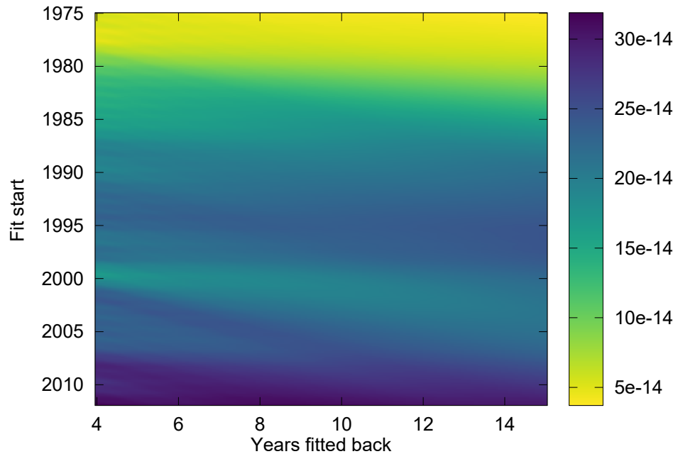
Coefficient b [ \text{mol mol}^{-1} \text{ years}^{-1} ]
