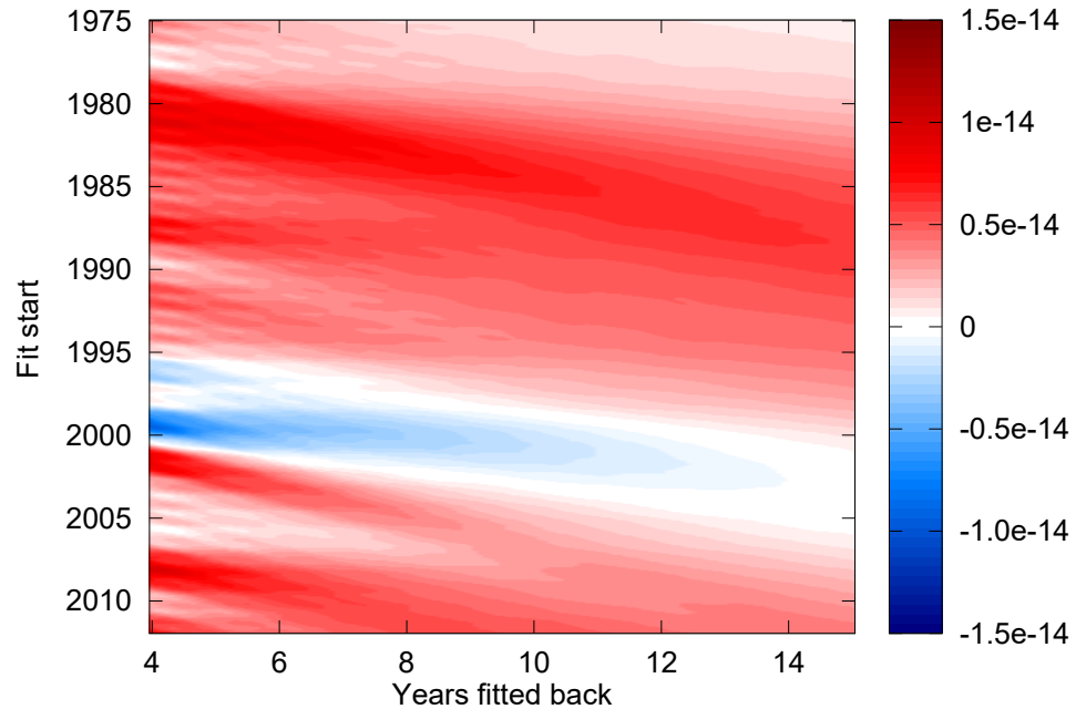
Coefficient c [ \text{mol mol}^{-1} \text{ years}^{-2} ]
