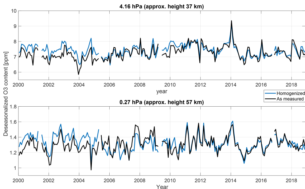
Figure 4. Deseasonalized ozone monthly mean time series before (in black) and after (in blue) the homogenization for a representative layer in the middle stratosphere and in the low mesosphere.
