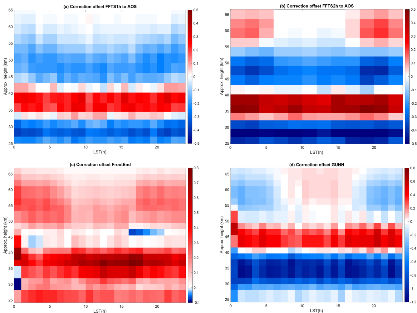
Figure 3. (a, b) Payerne MWR AOS setup vs. FFT setup offset profiles in parts per million as a function of LST; (c) correction offset for the front end (in 2005) and (d) for the GUNN oscillator (in 2009) technical upgrades.
