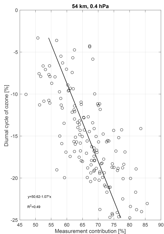
Figure 2. Ozone diurnal cycle amplitude (in percent of midnight value) as a function of measurement contribution (in percent of ozone content) for the lower mesosphere (0.4 hPa).
