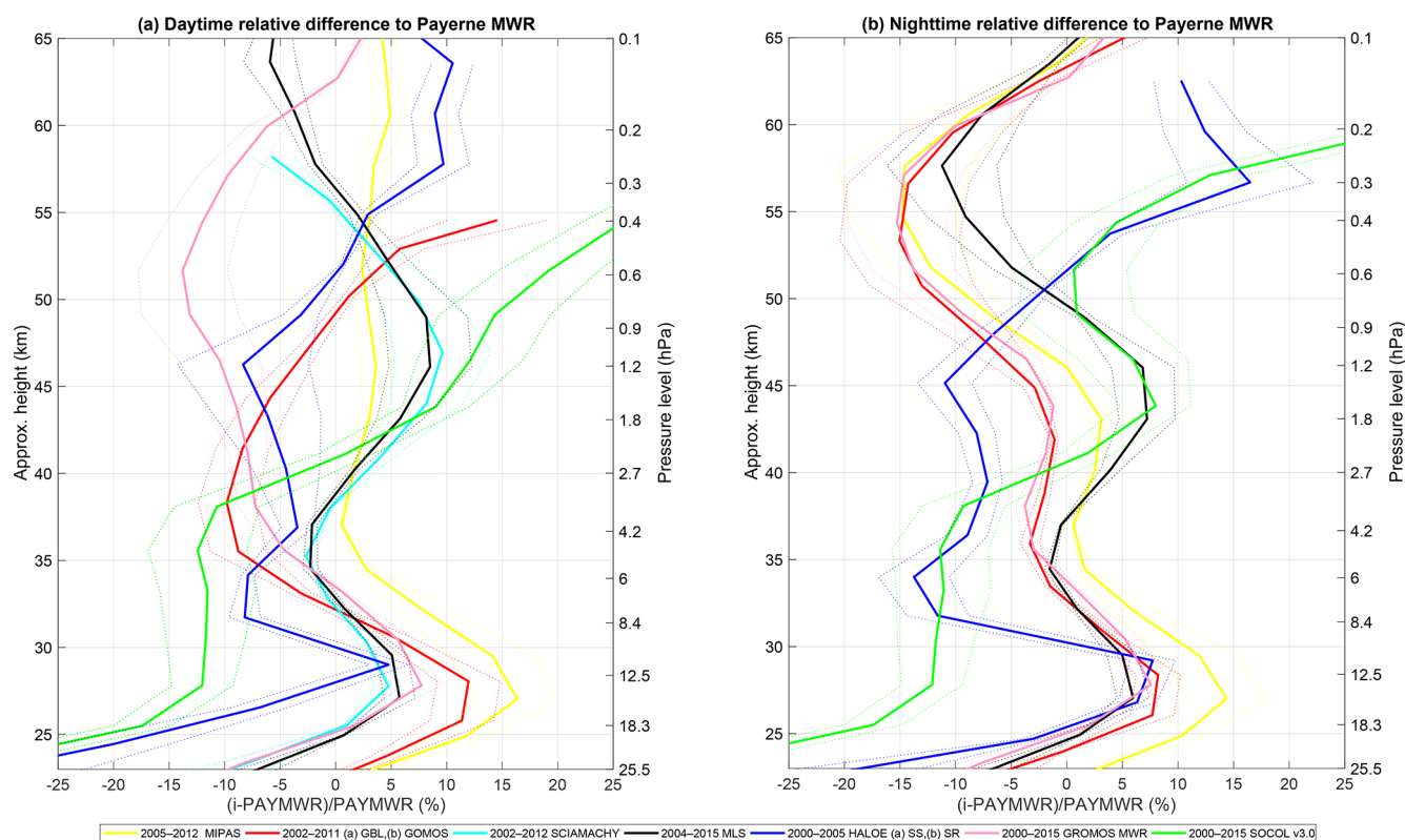
Figure 5. Payerne MWR bias vertical structure: mean of the relative difference between Payerne MWR and satellites MIPAS, MLS, GOMOS, GBL, SCIAMACHY, HALOE (a) SS and (b) SR and Bern MWR and SOCOL v3.0 CCM, for (a) daytime (10:00–14:00 LST) and (b) nighttime measurements (22:00–02:00 LST).
