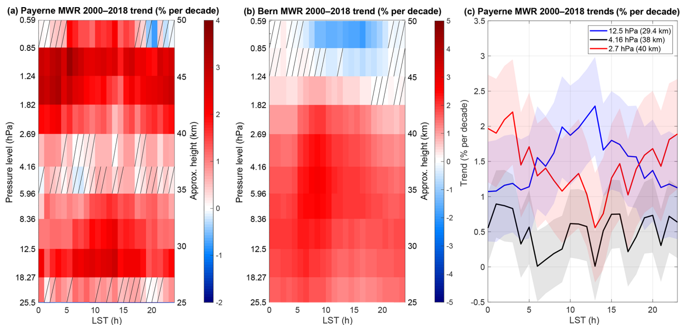
Figure 9. Long-term trends in percent per decade vs. LST for the 2000–2018 period. Trend estimates nonsignificantly different from zero at 95 % are hatched. (a) Payerne MWR 1 h time resolution dataset, (b) Bern MWR 1 h time resolution dataset and (c) Payerne MWR O 3 trends in percent per decade at 2.7 hPa (red), at morning minimum (12.5 hPa, blue) and at afternoon maximum (4.16 hPa, black) pressure levels vs. LST.
