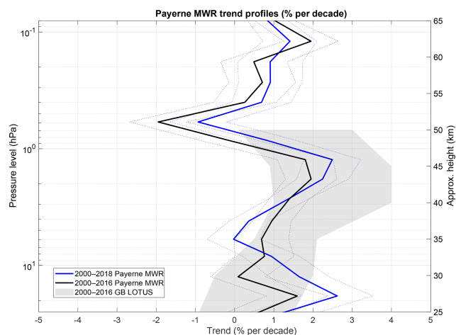
Figure 7. Payerne MWR O 3 trend profiles for the 2000–2016 time range in black and 2000–2018 time range in blue. The dotted lines show the 2\sigma uncertainties. The shaded area is the full range of LOTUS ground-based 2000–2016 trend profiles.
