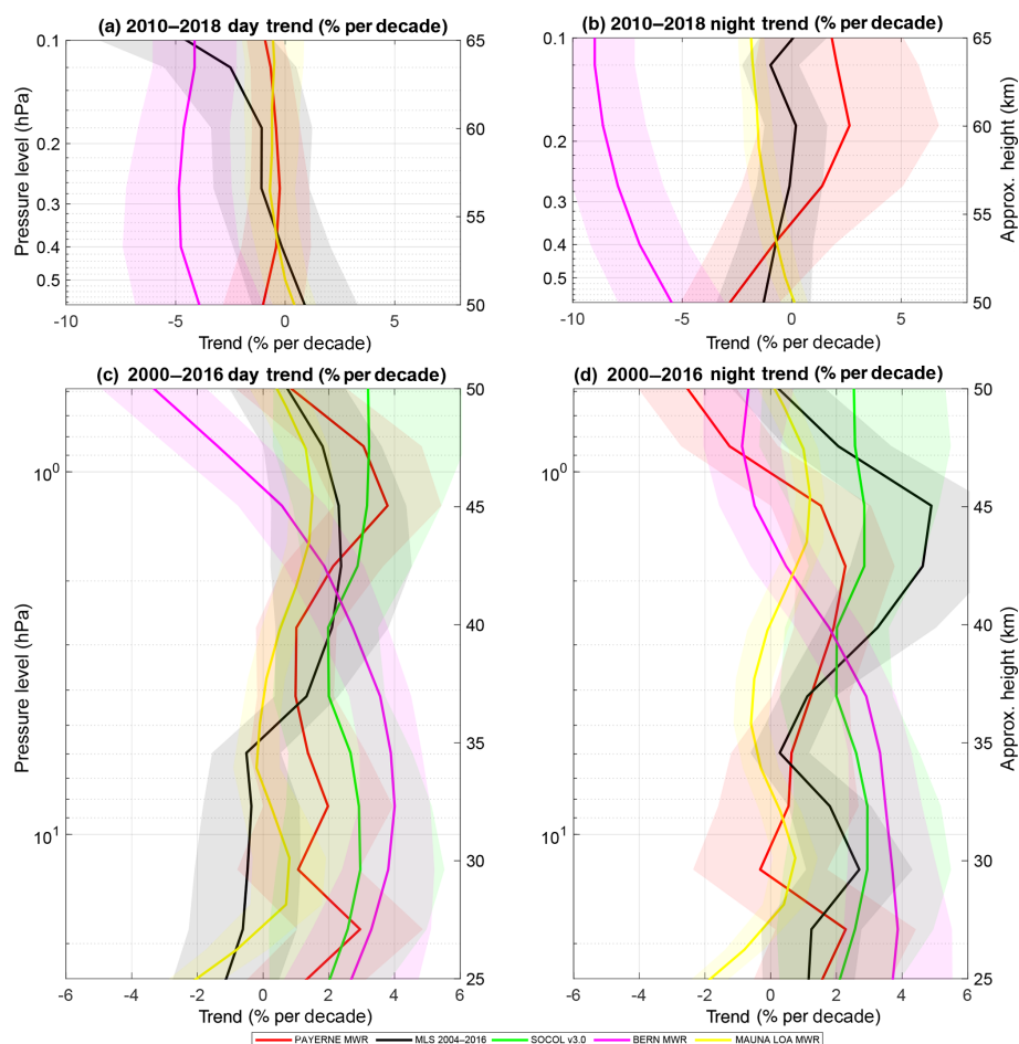
Figure 8. The 2000–2016 stratospheric (c, d) and 2010–2018 low-mesospheric (a, b) day- and nighttime trend profiles for Payerne MWR, MLS, SOCOL v3.0, Bern MWR and 2000–2015 MLO MWR. The shaded areas show the 2\sigma uncertainties.
