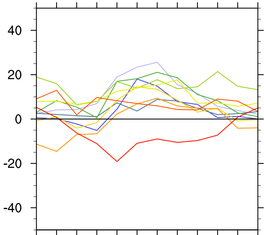
SW radiation
