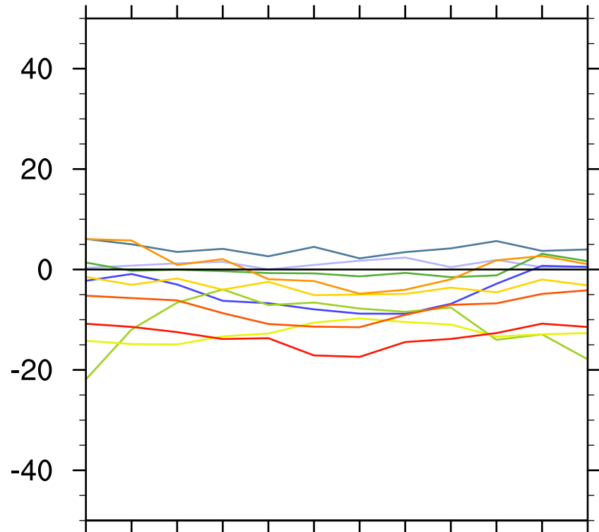
LW radiation
