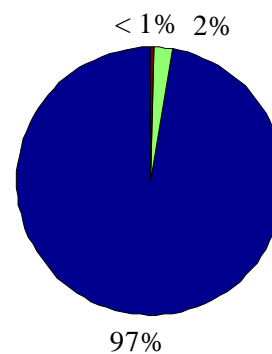
Daytime oxidation of unsaturated NMVOCs
