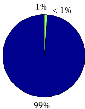
Nighttime oxidation of NMVOCs, CH 4 and CO
