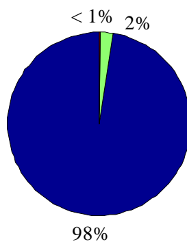
Daytime oxidation of NMVOCs
