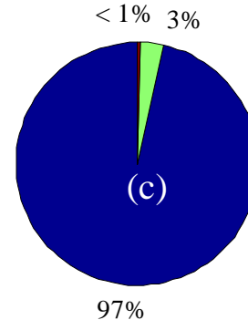
Daytime oxidation of unsaturated NMVOCs
