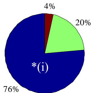
Nighttime oxidation of unsaturated NMVOCs
