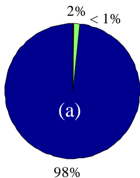
Daytime oxidation of NMVOCs, CH 4 and CO
