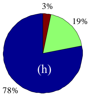
Nighttime oxidation of NMVOCs
