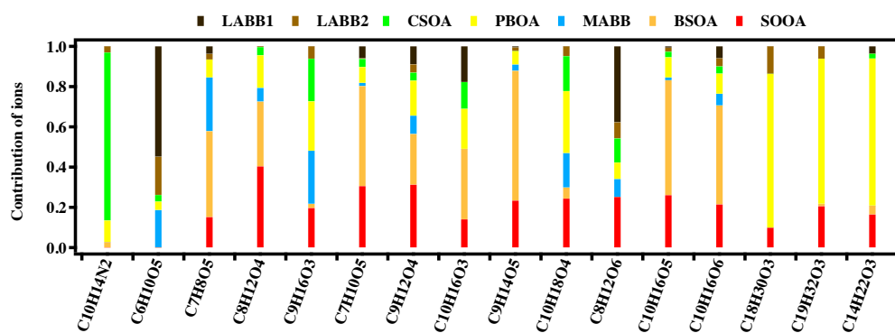
Fig. S12. Contribution of each ions to each factor from EESI-TOF PMF analysis.
