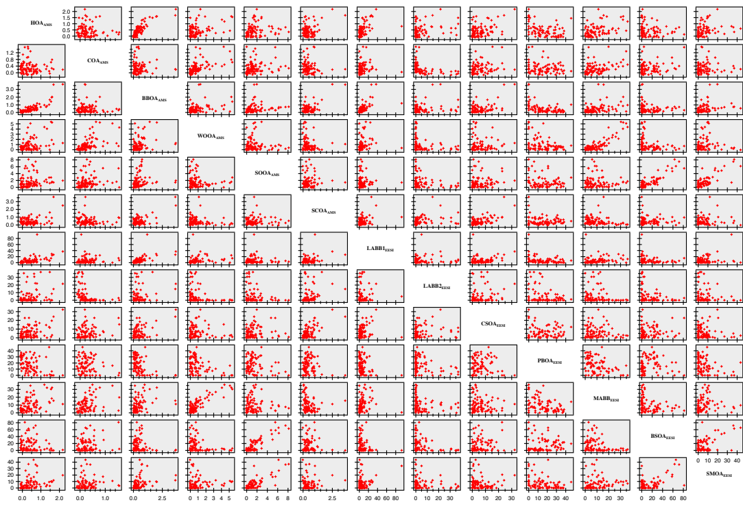
Fig. S13. Correlation between all the AMS and EESI factors.
