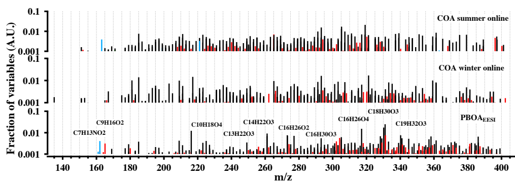
Fig. S10. The mass spectrum comparison between the PBOA factor and reference COA EESI factor (Qi et al., 2019, Stefenelli et al., 2019).
