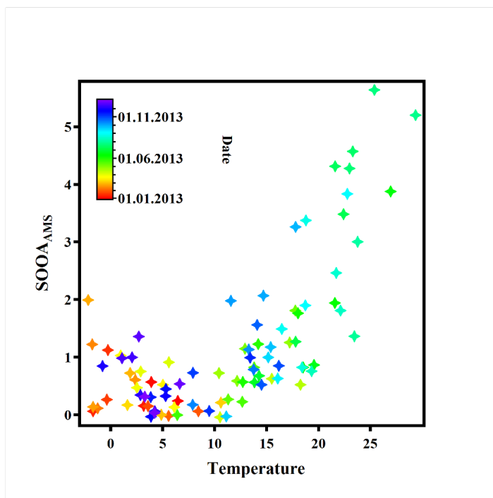
Fig. S11. The scatter plot of the temperature as a function of the SMOA EESI factor (a), BSOA EESI factor (b) and SOOA AMS factor of the EESI-TOF PMF.
