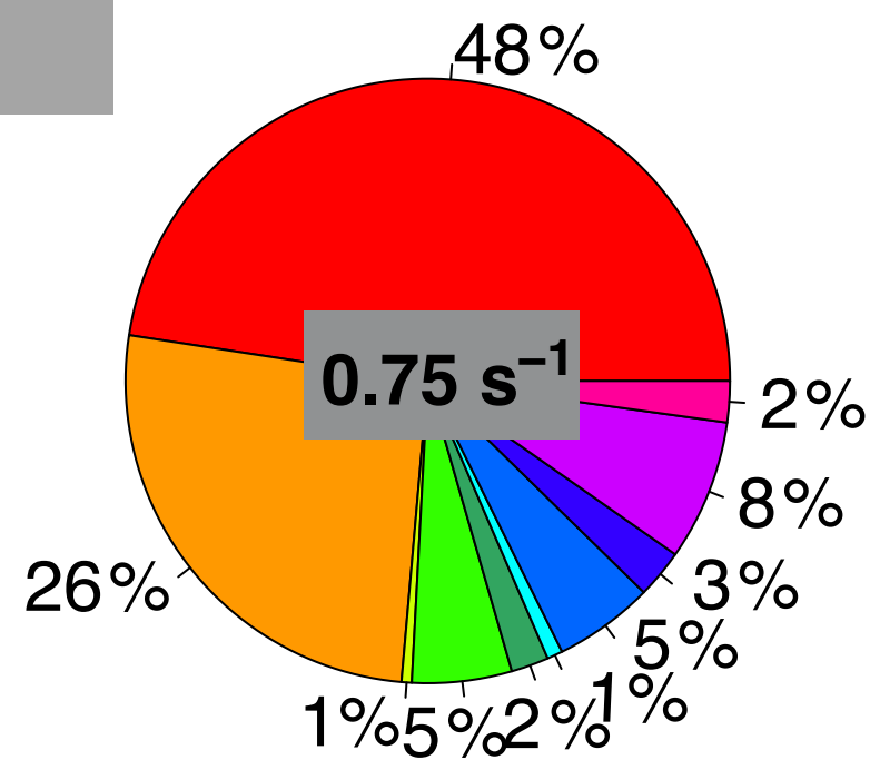
Model (SH)
