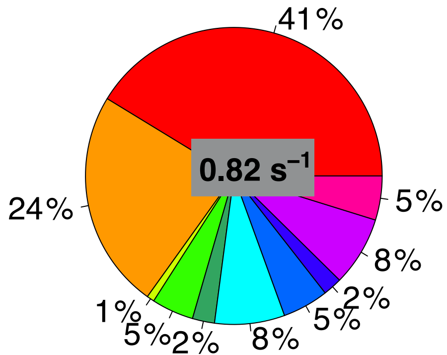
Observations (SH)
