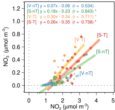
(b) \text{NO}_3^- vs. \text{NO}_2
