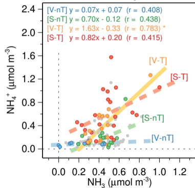
(c) \text{NH}_4^+ vs. \text{NH}_3
