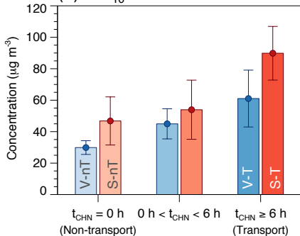
(e) PM 10
