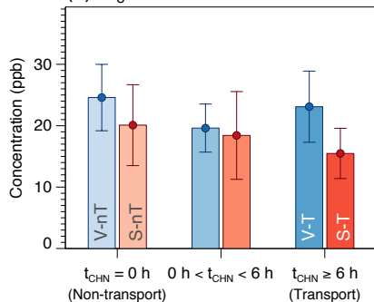
(c) O 3
