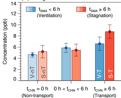
(a) SO 2
