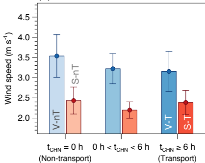
(c) WS
