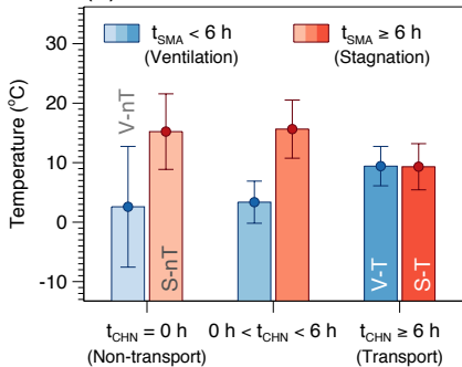
(a) T
