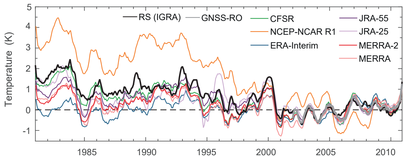
Temperature, pressure, and height anomalies, cold point tropopause
