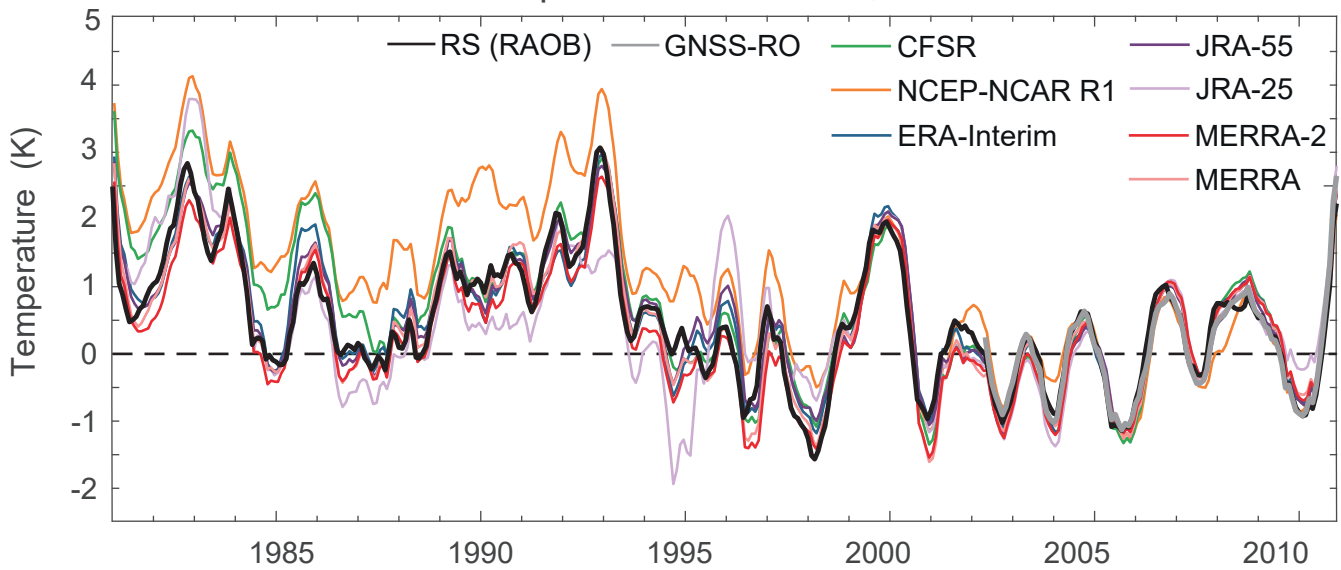
Temperature anomalies, 70 hPa
