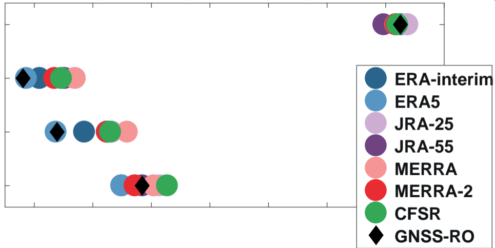
Temperature (20° S–20° N), 2002–2010
