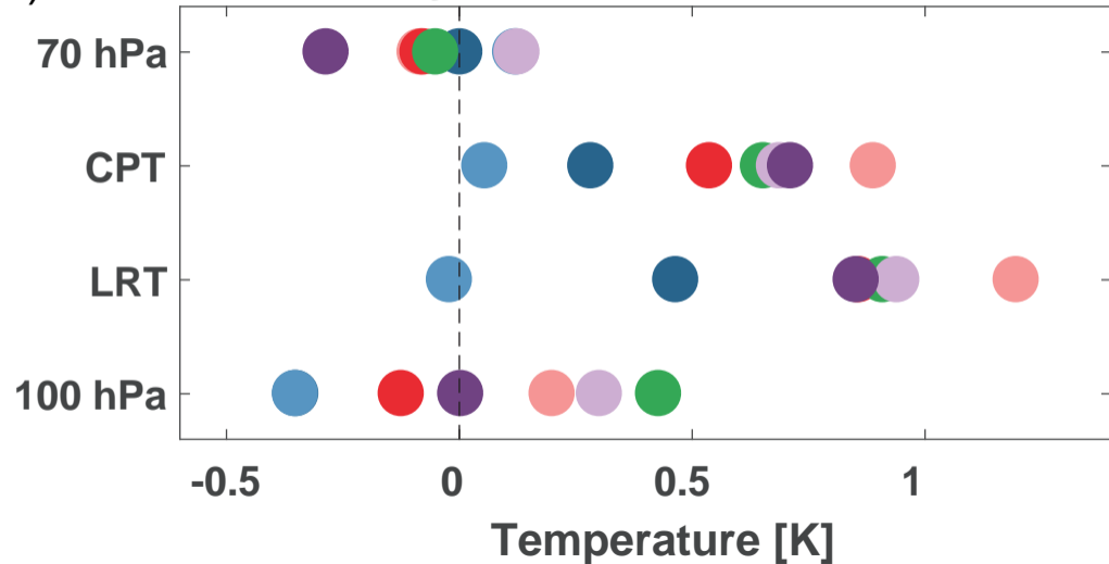
Reanalysis – GNSS-RO, 2002–2010
