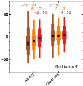
AERONET direct sun L2.0 AOT
