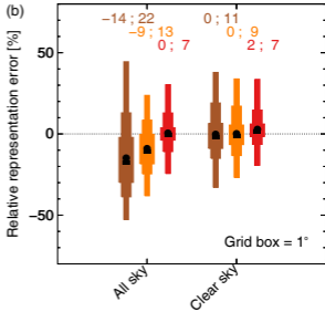
AERONET direct sun L2.0 AOT
