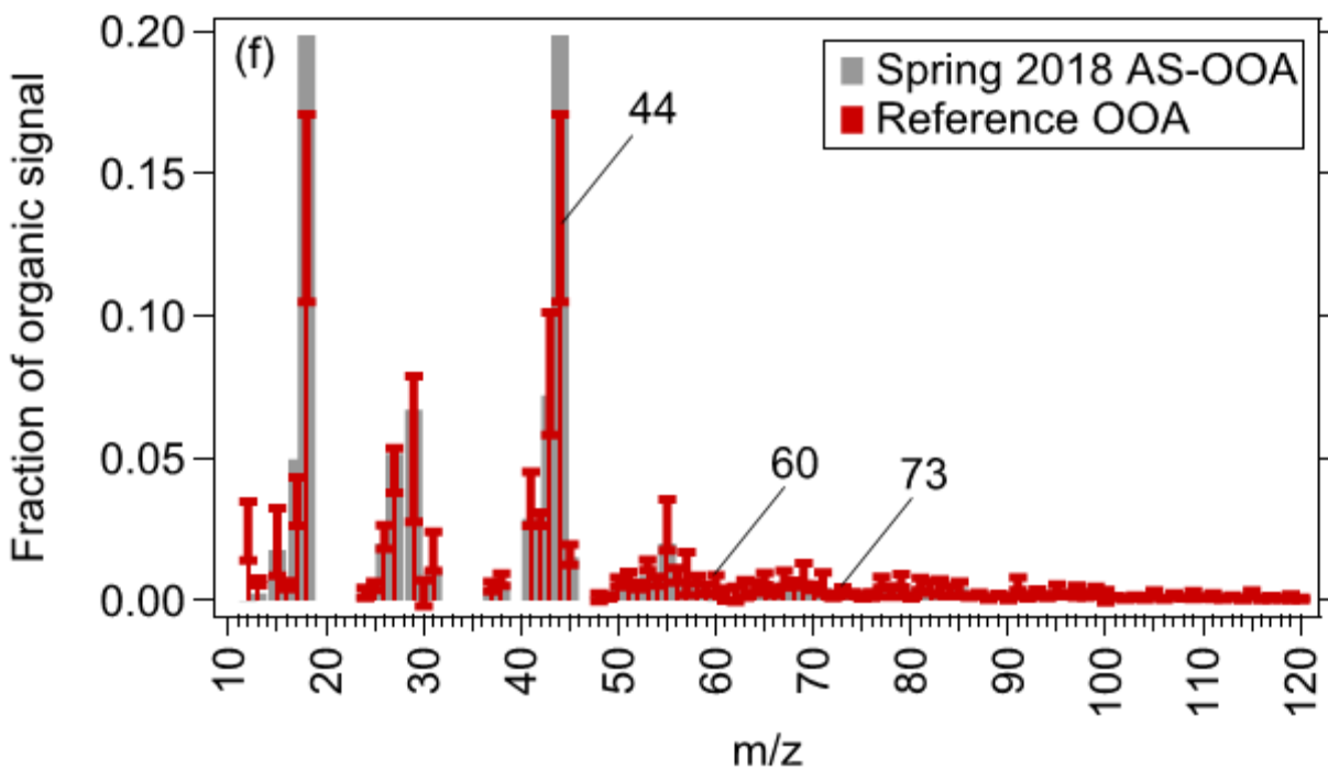
Figure S21 shows the mass spectrum of the organic component (AS-OOA) of the combined organic-inorganic PMF factor ammonium sulfate mixed with oxidized organic aerosol (ASOOA) in different seasons. The whiskers in the graphs represent \pm 1 standard deviation of the reference spectra. The comparison of PMF factor MS with reference OOA MS profile is shown in the order:
