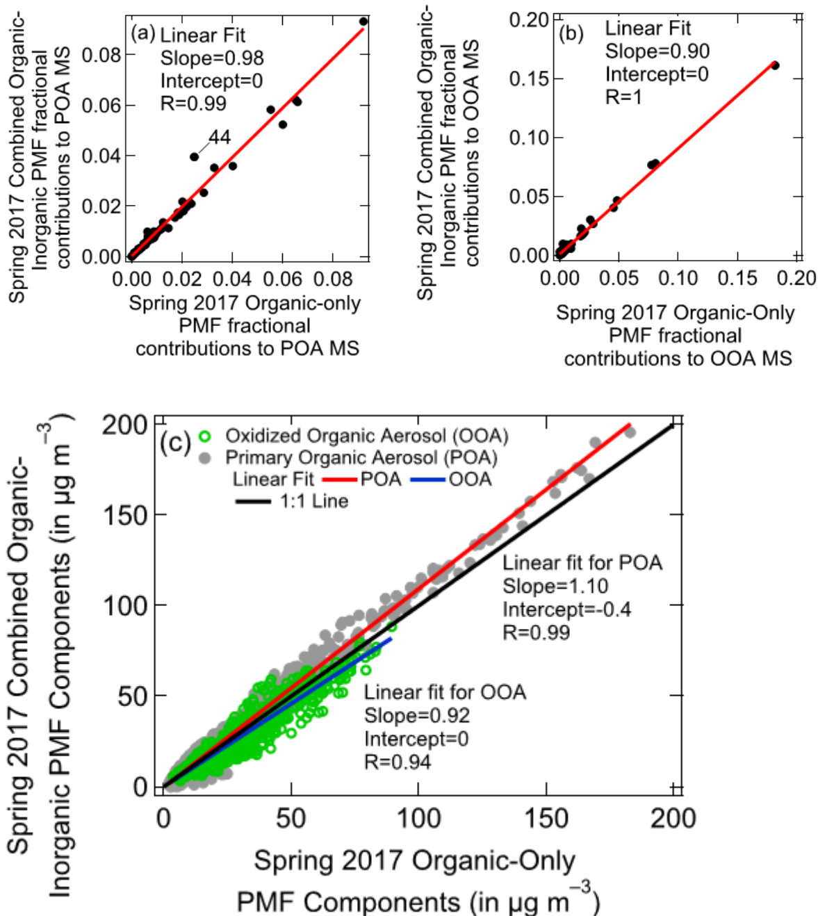
Figure S10 shows the comparison of combined organic-inorganic PMF and organic-only PMF MS for (a) the POA factor and (b) the OOA factor in spring 2017. Subplot (c) shows the comparison of combined organic-inorganic PMF and organic-only PMF-based factor concentrations ( \mu\text{g m}^{-3} ). The Pearson R coefficient indicates excellent linear correlations between the two analyses in all subplots. Based on the slope of the time series correlations, the combined organic-inorganic PMF estimates 10% more POA and about 8% less OOA than organic-only PMF in spring 2017.
