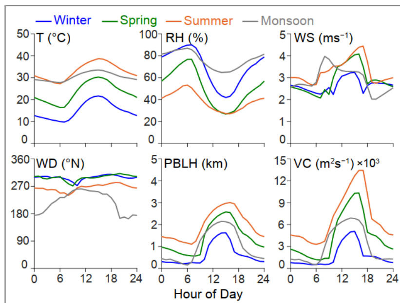
Figure S15 Diurnal profiles of meteorological parameters (temperature, relative humidity, wind speed, wind direction, PBLH, and VC) by season. Average values by season and hour of the day are presented for all parameters except wind direction. The median value is presented for wind direction. Ventilation coefficient (VC) = PBLH \times wind speed. Adapted from Gani et al. (2019).
