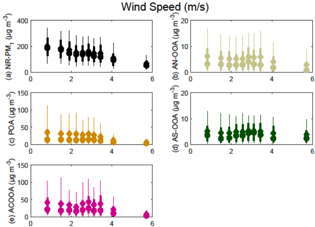
Figure S30 shows box plots of the PMF factor concentrations corresponding to deciles of wind speeds ( \text{ms}^{-1} ). The subplots correspond to concentrations ( \mu\text{g m}^{-3} ) of (a) NR-PM 1 , (b) AN-OOA, (c) POA, (d) AS-OOA, and (e) ACOOA. Note that ACOOA, in contrast to the other PMF factors, also include inorganic mass (which on average accounts for 80% of the ACOOA factor).
