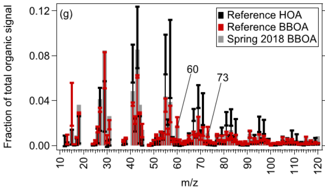
Figure S2 shows the mass spectrum of organic-only PMF mixed hydrocarbon-like organic aerosol (HOA)-biomass burning organic aerosol (BBOA) (POA) factor in different seasons, which is similar to the reference HOA and BBOA factors. The whiskers in the graphs represent \pm 1 standard deviation of the reference spectra. The comparison of PMF factor MS with reference profiles is shown in the order: (a) winter 2017 POA, (b) spring 2017 POA, (c) summer 2017 POA, (d) monsoon 2017 POA, (e) winter 2018 POA, (f) spring 2018 HOA, and (g) spring 2018 BBOA. The profiles show the influence of both HOA and BBOA-type aerosols.
