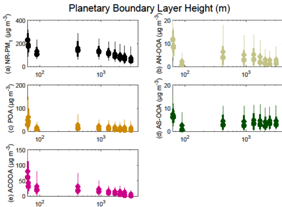
Figure S31 shows box plots of the PMF factor concentrations corresponding to deciles of planetary boundary layer height (m). The subplots correspond to concentrations ( \mu\text{g m}^{-3} ) of (a) NR-PM 1 , (b) AN-OOA, (c) POA, (d) AS-OOA, and (e) ACOOA. Note that the x-axes in the subplots
