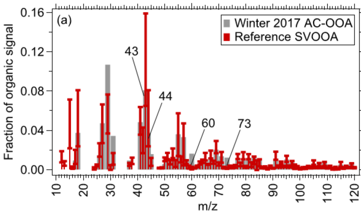
Figure S24 shows box plots of the PMF factor concentrations corresponding to deciles of relative humidity (%). The subplots correspond to concentrations ( \mu\text{g m}^{-3} ) of (a) NR-PM 1 , (b) AN-OOA, (c) POA, (d) AS-OOA, and (e) ACOOA. Note that ACOOA, in contrast to the other PMF factors, also include inorganic mass (which on average accounts for 80% of the ACOOA factor).
