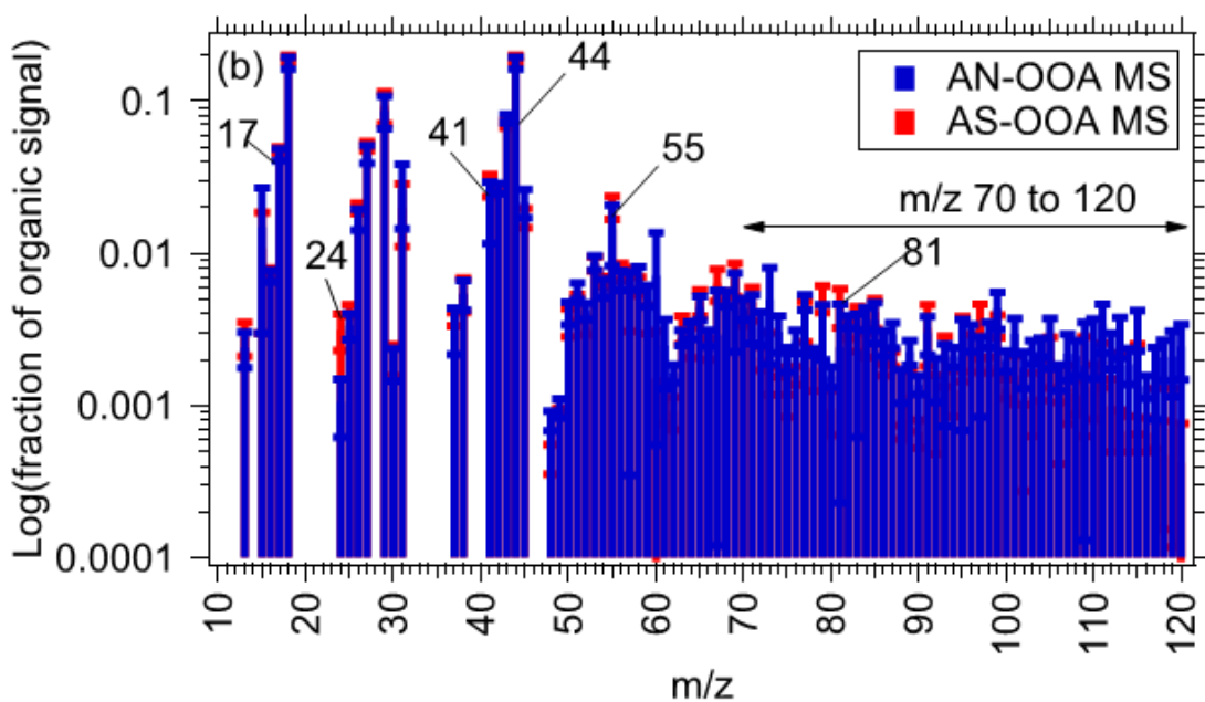
Figure S23 shows the comparison of logarithmic fractional contributions at different m/z s in the organic components AN-OOA and AS-OOA of the combined organic-inorganic PMF factors ANOOA and ASOOA with (a) AS-OOA overlaid on AN-OOA and (b) AN-OOA overlaid on AS-OOA. AS-OOA profiles have a higher contribution at prominent lower m/z s, such as 17, 24, 41, 44, 55, and 81. AN-OOA has higher contribution at m/z 43 and at higher m/z s between 70–120.
