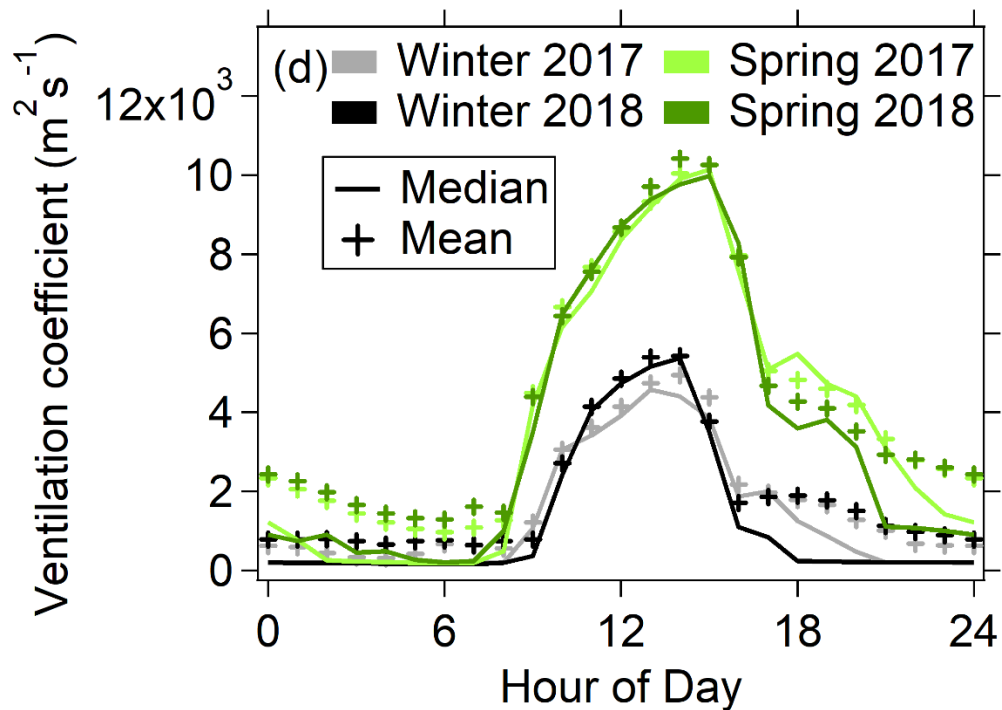
Figure S29 This figure shows the diurnal patterns of mean and median (a) relative humidity (%), (b) temperature (°C), (c) wind direction (°), (d) ventilation coefficient ( \text{m}^2 \text{s}^{-1} ) across winters and springs of 2017 and 2018.
