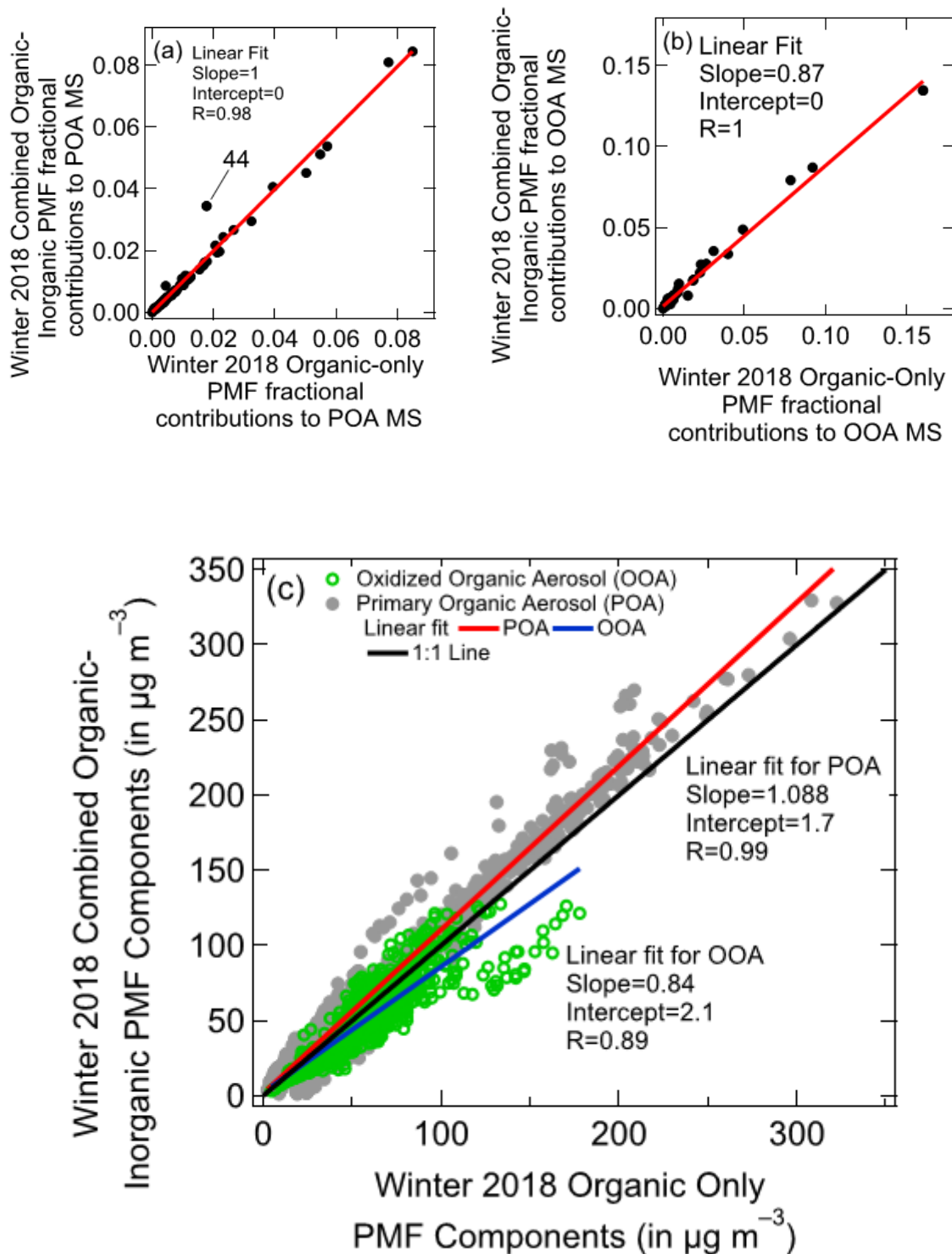
Figure S13 shows the comparison of combined organic-inorganic PMF and organic-only PMF MS for (a) the POA factor and (b) the OOA factor in winter 2018. Subplot (c) shows the comparison of combined organic-inorganic PMF and organic-only PMF-based factor concentrations ( \mu\text{g m}^{-3} ). The Pearson R coefficient indicates excellent linear correlations between the two analyses in all subplots. Based on the slope of the time series correlations, the combined organic-inorganic PMF estimates about 9% more POA and 16% less OOA than organic-only PMF in winter 2018.
