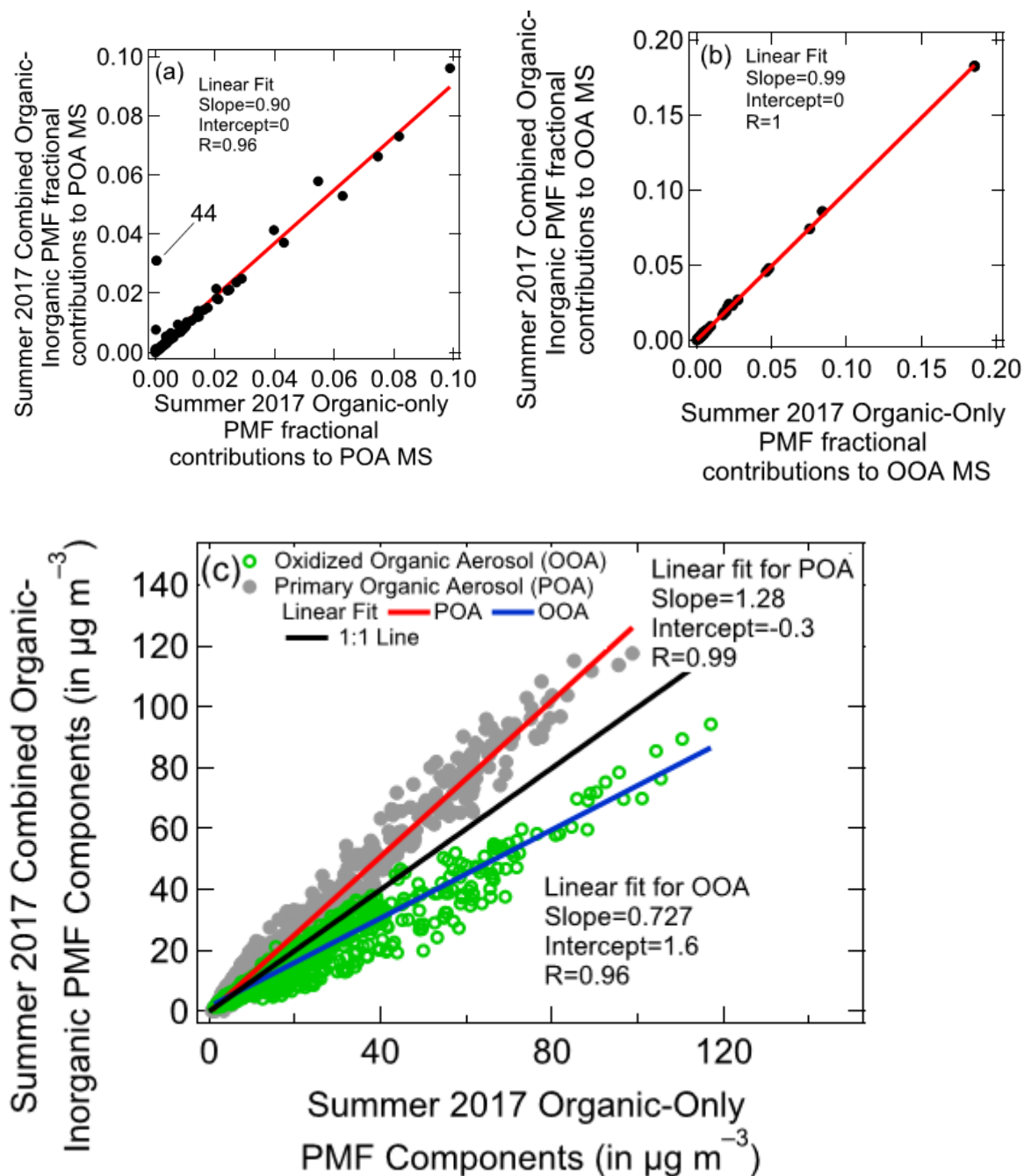
Figure S11 shows the comparison of combined organic-inorganic PMF and organic-only PMF MS for (a) the POA factor and (b) the OOA factor in summer 2017. Subplot (c) shows the comparison of combined organic-inorganic PMF and organic-only PMF-based factor concentrations ( \mu\text{g m}^{-3} ). The Pearson R coefficient indicates excellent linear correlations between the two analyses in all subplots. Based on the slope of the time series correlations, the combined organic-inorganic PMF estimates 28% more POA and about 27% less OOA than organic-only PMF in summer 2017.
