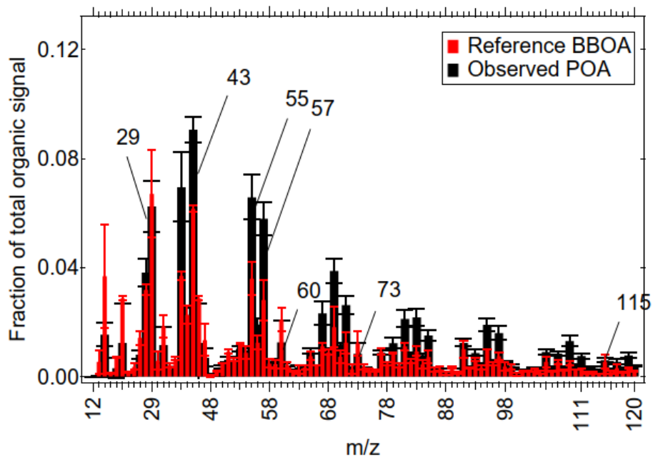
Figure S3 This figure shows the average mass spectrum of the organic-only PMF primary organic aerosol (POA) factor. At m/z s 29, 60, 73 and 115, observed POA signals are in line with the reference biomass burning organic aerosol (BBOA) factor.
