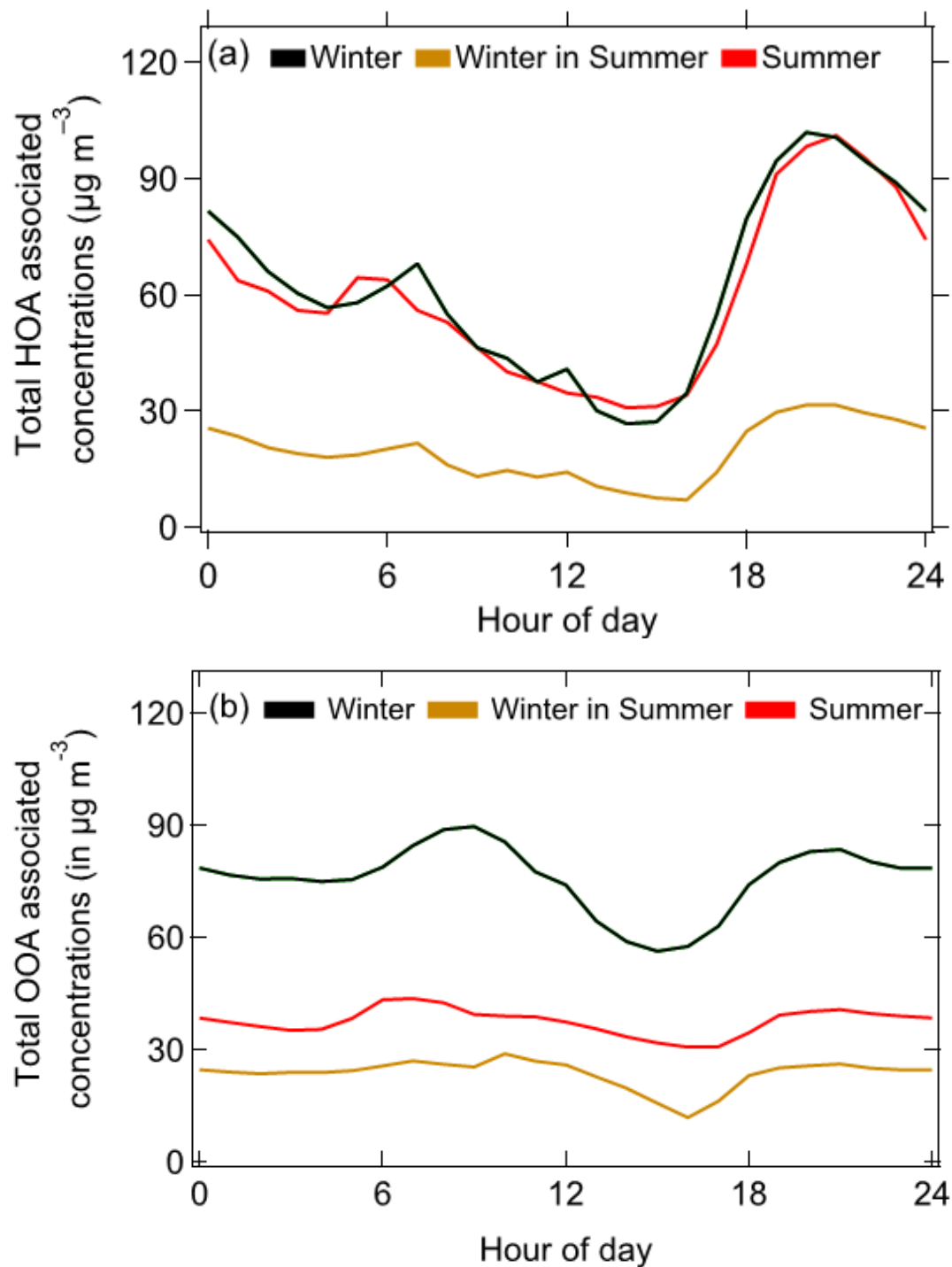
Figure S17 This figure shows the diurnal variations of (a) total HOA-associated concentrations, (b) total OOA-associated concentrations. Application of VBS to winter and summer diurnal averaged data generates very similar diurnal variations in total HOA-associated concentrations. In contrast, total OOA-associated concentrations have halved between winter and summer and have flatter diurnal variations.
