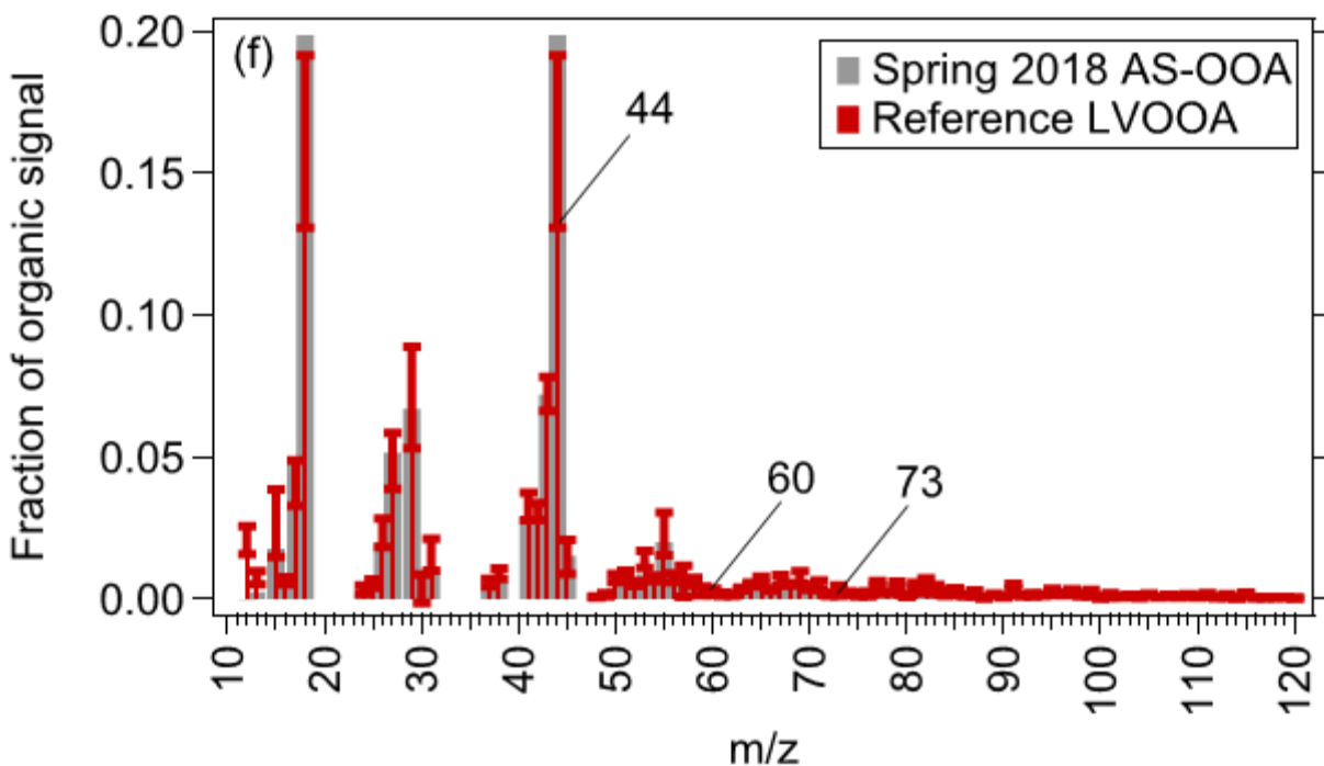
Figure S22 shows the mass spectrum of the organic component (AS-OOA) of the combined organic-inorganic PMF factor ammonium sulfate mixed with oxidized organic aerosol (ASOOA) in different seasons, which is similar to the reference LVOOA MS profile. The whiskers in the graphs represent \pm 1 standard deviation of the reference spectra. The comparison of PMF factor MS with reference profiles is shown in the order: (a) winter 2017, (b) spring 2017, (c) summer 2017, (d) monsoon 2017, (e) winter 2018, and (f) spring 2018.
