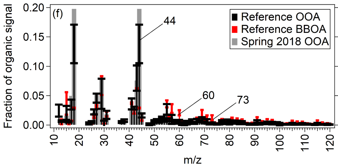
Figure S5 shows the mass spectrum of organic-only PMF oxidized organic aerosol (OOA) factor in different seasons, which is similar to the reference OOA factor. The whiskers in the graphs represent \pm 1 standard deviation of the reference spectra. The comparison of PMF factor MS with reference profiles is shown in the order: (a) winter 2017, (b) spring 2017, (c) summer 2017, (d) monsoon 2017, (e) winter 2018, and (f) spring 2018. MS in most seasons are marked by a higher contribution at m/z 44 than the reference OOA profile, pointing to the highly oxidized nature of aerosols.
