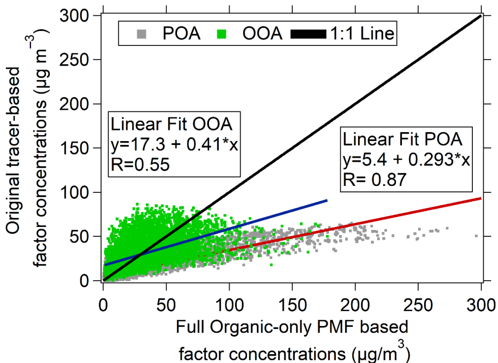
Figure S27 shows the comparison of the tracer-based OOA and POA concentrations with those obtained from organic-only PMF, without the application of mass closure. The linear correlations and slopes are substantially different from 1 and point to the limitation of this tracer approach.
