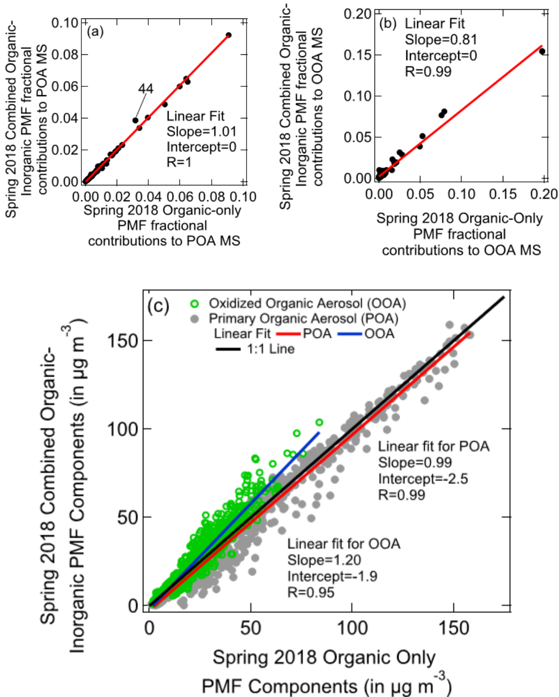
Figure S14 shows the comparison of combined organic-inorganic PMF and organic-only PMF MS for (a) the POA factor and (b) the OOA factor in spring 2018. Subplot (c) shows the comparison of combined organic-inorganic PMF and organic-only PMF-based factor concentrations ( \mu\text{g m}^{-3} ). The Pearson R coefficient indicates excellent linear correlations between the two analyses in all subplots. Based on the slope of the time series correlations, the combined organic-inorganic PMF estimates about 1% less POA and 20% more OOA than organic-only PMF in spring 2018.
