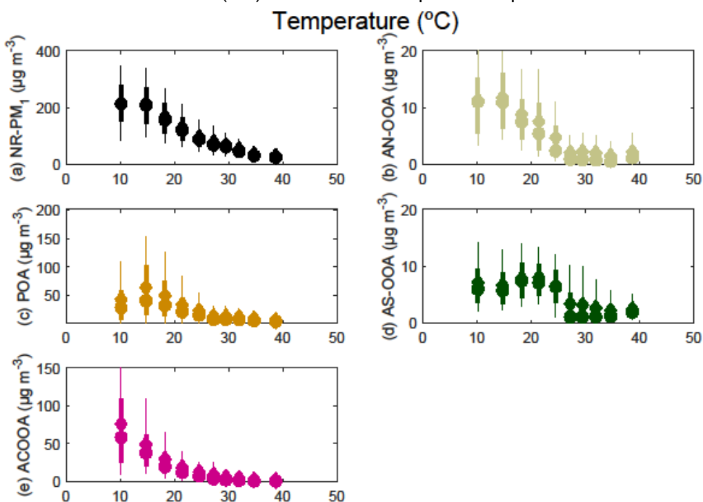
Figure S16 shows box plots of the PMF factor concentrations corresponding to deciles of temperature ( ^{\circ}\text{C} ). The subplots correspond to concentrations ( \mu\text{g m}^{-3} ) of (a) NR-PM 1 , (b) AN-OOA, (c) POA, (d) AS-OOA, and (e) ACOOA. Note that ACOOA, in contrast to the other PMF factors, also include inorganic mass (which on average accounts for 80% of the ACOOA factor).
