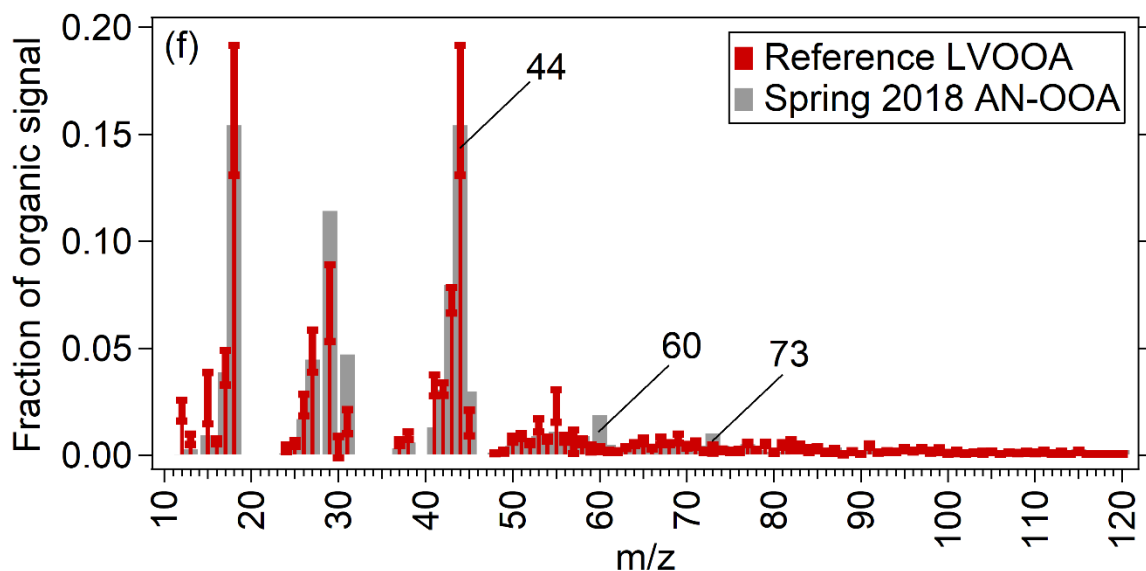
Figure S20 shows the mass spectrum of the organic component (AN-OOA) of the combined organic-inorganic PMF factor ammonium nitrate mixed with oxidized organic aerosol (ANOOA) in different seasons. The whiskers in the graphs represent \pm 1 standard deviation of the reference spectra. The comparison of PMF factor MS with the reference MS profile of LVOOA is shown in the order: (a) winter 2017, (b) spring 2017, (c) summer 2017, (d) monsoon 2017, (e) winter 2018, and (f) spring 2018. The AN-OOA MS is similar to the reference LVOOA profile.
