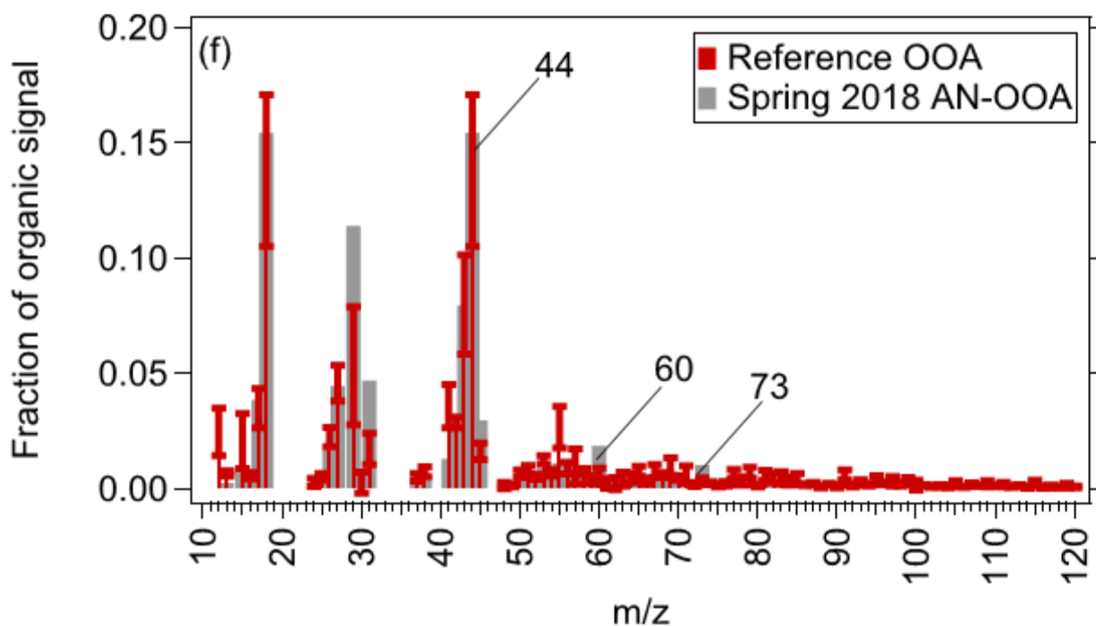
Figure S19 shows the mass spectrum of the organic component (AN-OOA) of the combined organic-inorganic PMF factor ammonium nitrate mixed with oxidized organic aerosol (ANOOA) in different seasons. The whiskers in the graphs represent \pm 1 standard deviation of the reference spectra. The comparison of PMF factor MS with the reference MS profile of OOA is shown in the order: (a) winter 2017, (b) spring 2017, (c) summer 2017, (d) monsoon 2017, (e) winter 2018, and (f) spring 2018. Clearly, the AN-OOA mass spectral profile is similar to reference OOA.
