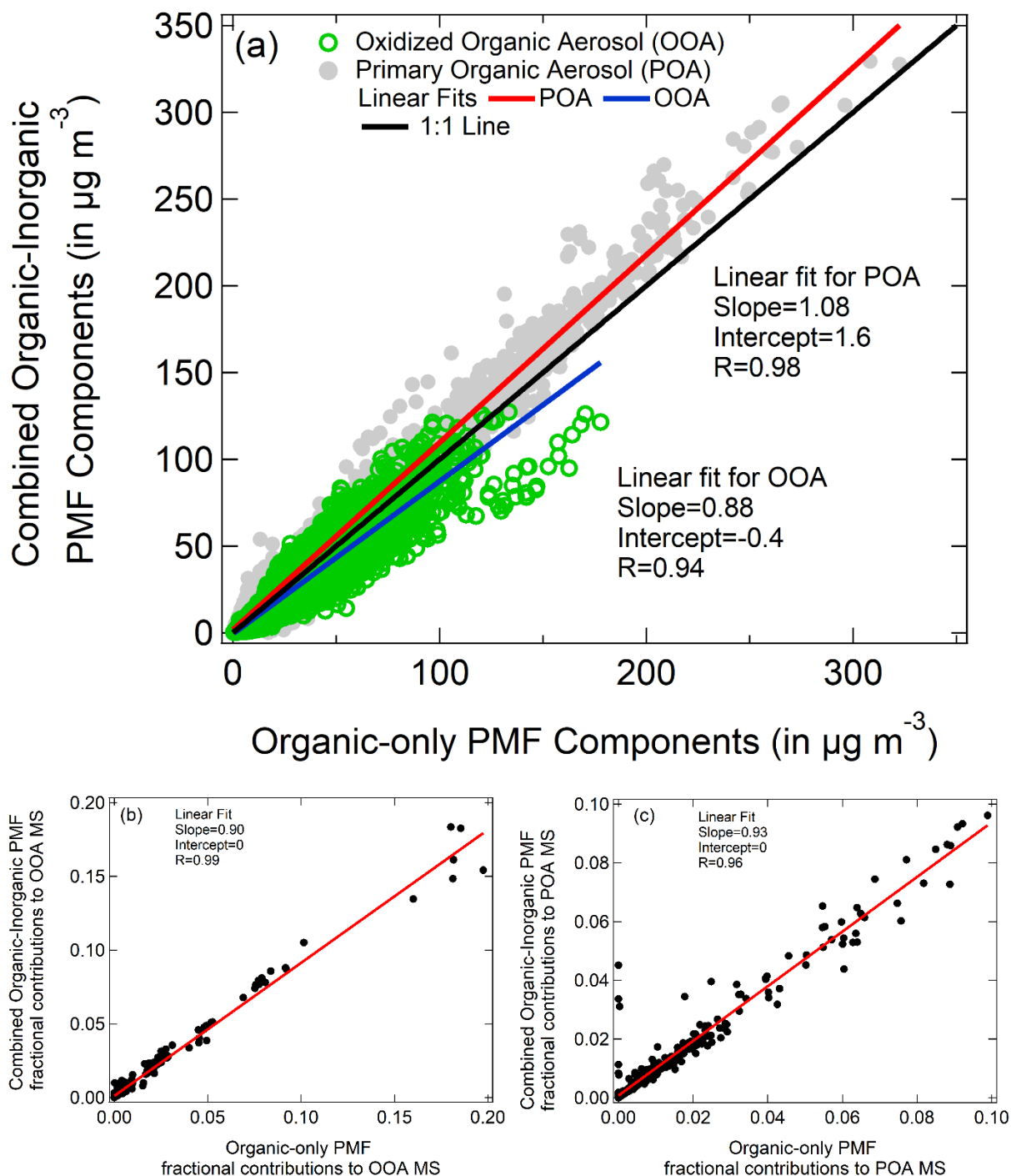
Figure S8 (a) Time series correlation of POA and OOA from combined organic-inorganic PMF and organic-only PMF analysis ( \mu\text{g m}^{-3} ) b) and c) Mass spectral correlations of the average OOA MS and POA MS from combined organic-inorganic PMF and organic-only PMF analysis. Strong correlations suggest an agreement between the analyses.
