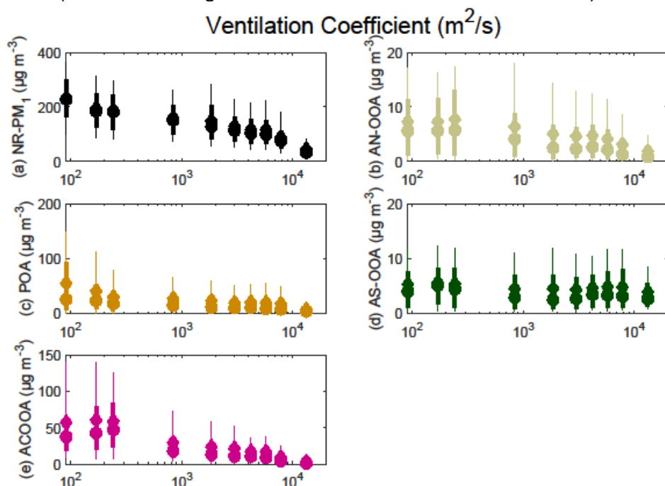
Figure S32 shows box plots of the PMF factor concentrations corresponding to deciles of ventilation coefficient ( m^2s^{-1} ). The subplots correspond to concentrations ( \mu g m^{-3} ) of (a) NR-PM 1 , (b) AN-OOA, (c) POA, (d) AS-OOA, and (e) ACOOA. Note that the x-axes in the subplots are on a logarithmic scale, and that ACOOA, in contrast to the other PMF factors, also include inorganic mass (which on average accounts for 80% of the ACOOA factor).
