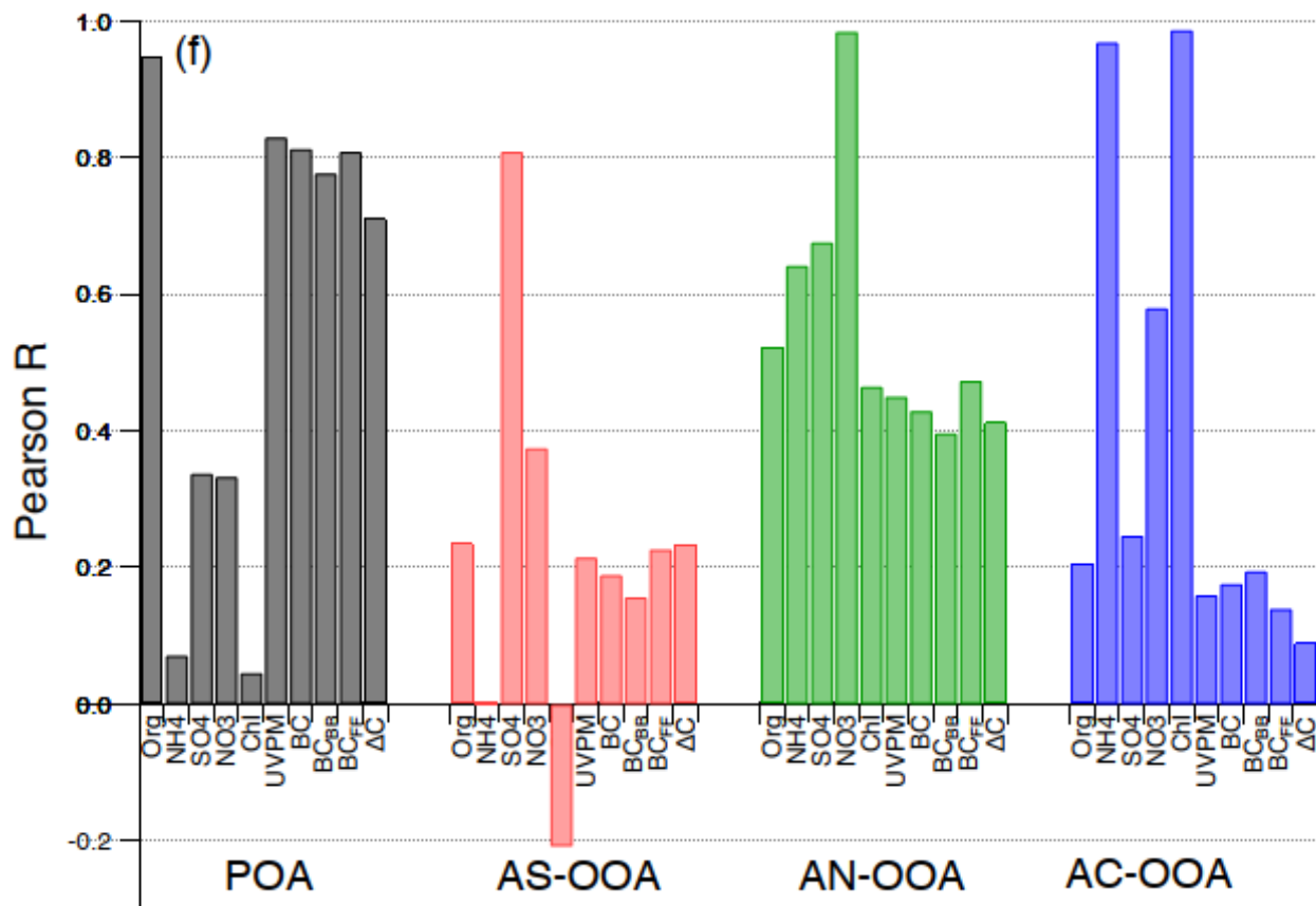
Figure S6 shows the time series correlations of the combined organic-inorganic PMF factors (or, their organic components—time series correlations within each season are, by definition, equal for the PMF factor and its organic component) with tracer species in different seasons. The comparison of PMF factors with tracers is shown in the order: (a) winter 2017, (b) spring 2017, (c) summer 2017, (d) monsoon 2017, (e) winter 2018, and (f) spring 2018. Clearly, AC-OOA (or, ACOOA) does not correlate with biomass burning tracers BC BB and ΔC.
