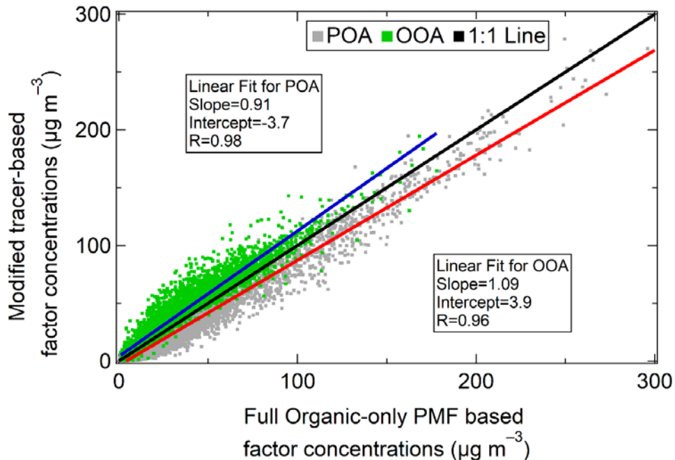
Figure S28 This figure shows the comparison of the modified tracer-based OOA and POA concentrations with those obtained from organic-only PMF. The strong linear correlations and slopes close to 1 point to the usefulness of the tracer approach for real-time source apportionment.
