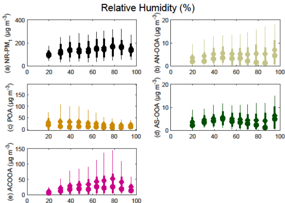
Figure S24 shows box plots of the PMF factor concentrations corresponding to deciles of relative humidity (%). The subplots correspond to concentrations ( \mu\text{g m}^{-3} ) of (a) NR-PM 1 , (b) AN-OOA, (c) POA, (d) AS-OOA, and (e) ACOOA. Note that ACOOA, in contrast to the other PMF factors, also include inorganic mass (which on average accounts for 80% of the ACOOA factor).
