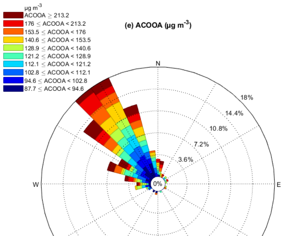
Figure S26 shows wind rose plots (indicating concentration by direction as opposed to the conventional wind rose plots that show wind speed by direction) corresponding to >90^{\text{th}} percentile concentrations of all PMF factors. Color scale corresponds to ten groups with equal numbers of observations: 1% each of the full observational dataset, and equivalently 10% each of the >90^{\text{th}} percentile observations. The subplots correspond to concentrations ( \mu\text{g m}^{-3} ) of (a) NR-PM 1 , (b) AN-OOA, (c) POA, (d) AS-OOA, and (e) ACOOA. Note that ACOOA, in contrast to the other PMF factors, also include inorganic mass (which on average accounts for 80% of the ACOOA factor).
