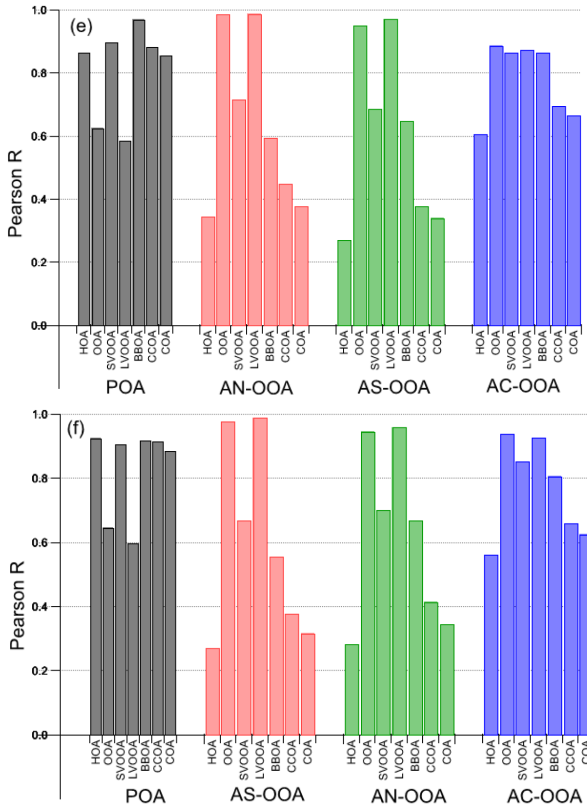
Figure S7 shows the correlations of the organic component MS of the combined organic-inorganic PMF factor with reference profiles in the order: (a) winter 2017, (b) spring 2017, (c) summer 2017, (d) monsoon 2017, (e) winter 2018, and (f) spring 2018. Clearly, all PMF factors show strong
