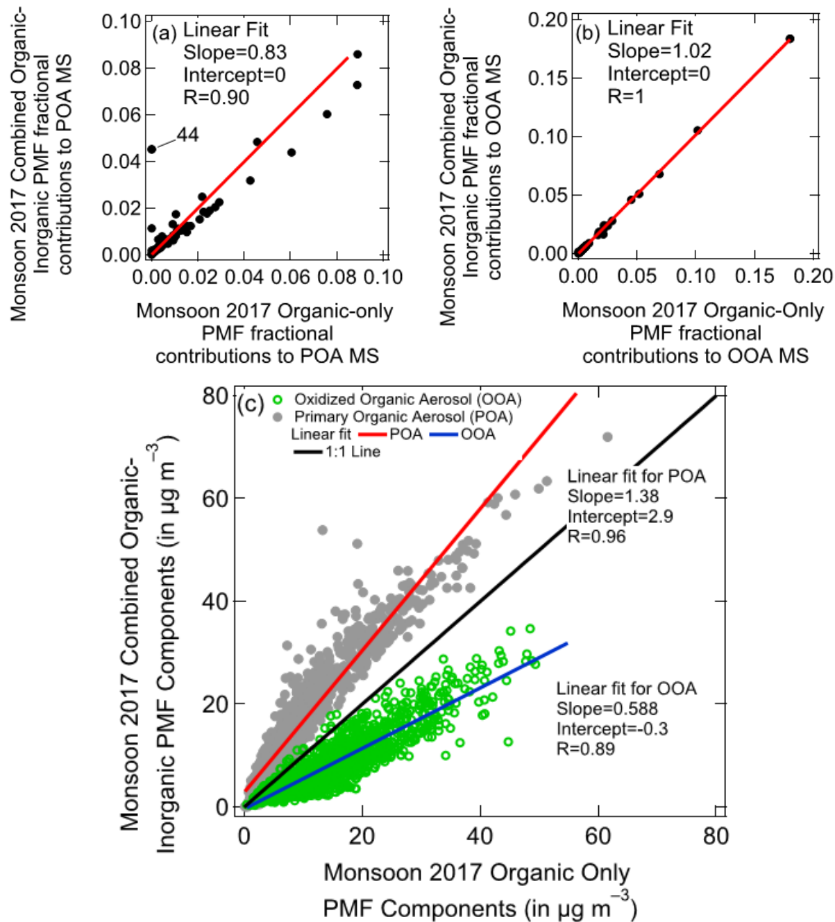
Figure S12 shows the comparison of combined organic-inorganic PMF and organic-only PMF MS for (a) the POA factor and (b) the OOA factor in monsoon 2017. Subplot (c) shows the comparison of combined organic-inorganic PMF and organic-only PMF-based factor concentrations ( \mu\text{g m}^{-3} ). The Pearson R coefficient indicates excellent linear correlations between the two analyses in all subplots. Based on the slope of the time series correlations, the combined organic-inorganic PMF estimates 38% more POA and about 41% less OOA than organic-only PMF in monsoon 2017.
