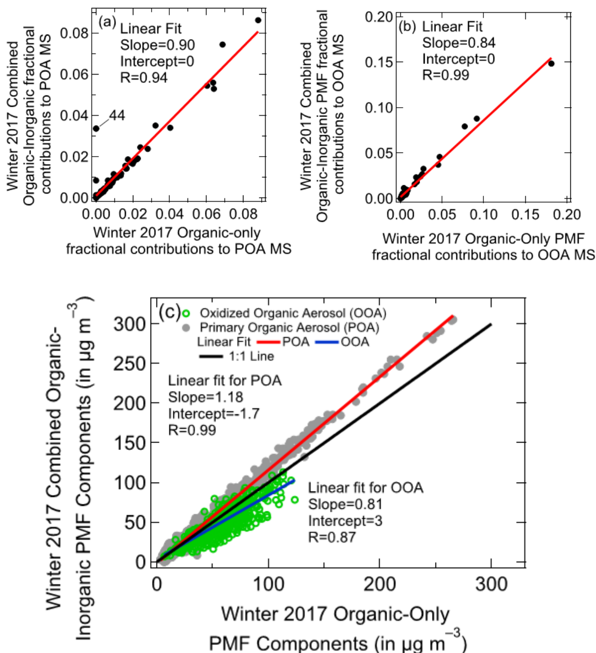
Figure S9 shows the comparison of combined organic-inorganic PMF and organic-only PMF MS for (a) the POA factor and (b) the OOA factor in winter 2017. Subplot (c) shows the comparison of combined organic-inorganic PMF and organic-only PMF-based factor concentrations ( \mu\text{g m}^{-3} ). The Pearson R coefficient indicates excellent linear correlations between the two analyses in all subplots. Based on the slope of the time series correlations, the combined organic-inorganic PMF estimates 18% more POA and about 19% less OOA than organic-only PMF in winter 2017.
