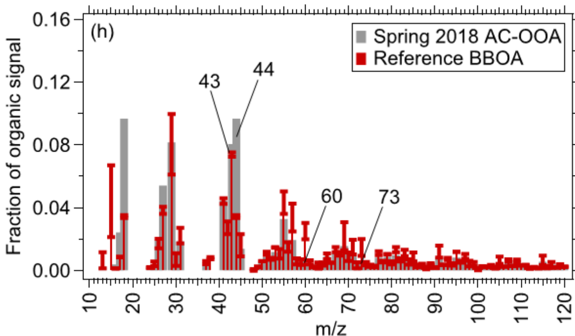
Figure S25 shows the mass spectrum of the organic component (AC-OOA) of the combined organic-inorganic PMF factor ammonium chloride mixed with oxidized organic aerosol (ACOOA) in different seasons, which shows similarities to the reference SVOOA and BBOA factors. The whiskers in the graphs represent \pm 1 standard deviation of the reference spectra. The comparison of the AC-OOA factor MS with the SVOOA reference profile are in the order: (a) winter 2017, (b) spring 2017, (c) winter 2018, and (d) spring 2018. The comparison of AC-OOA factor MS with the BBOA reference profile are in the order: (e) winter 2017, (f) spring 2017, (g) winter 2018, and (h) spring 2018. These figures show that the factors resemble oxidized biomass burning aerosol (higher fraction of organics at m/z s 60 and 73 than reference OOA profile).
