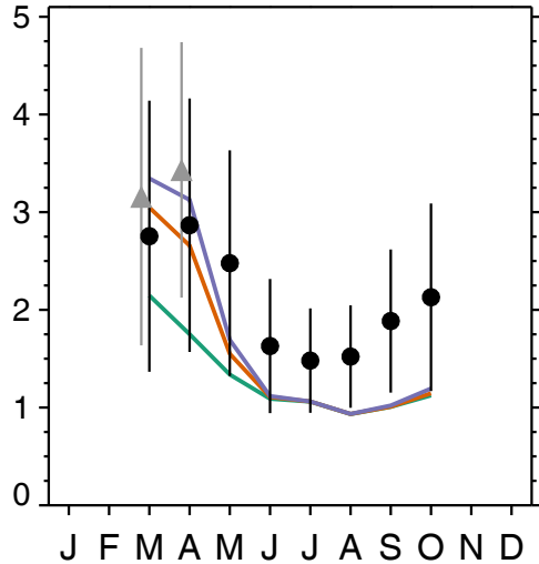
(c) 60–90° N
