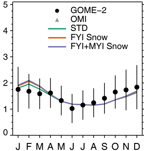
(b) 30–60° N
