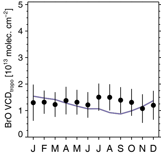
(a) 0–30° N
