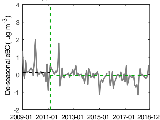
(c) eBC mass concentration at LTR
