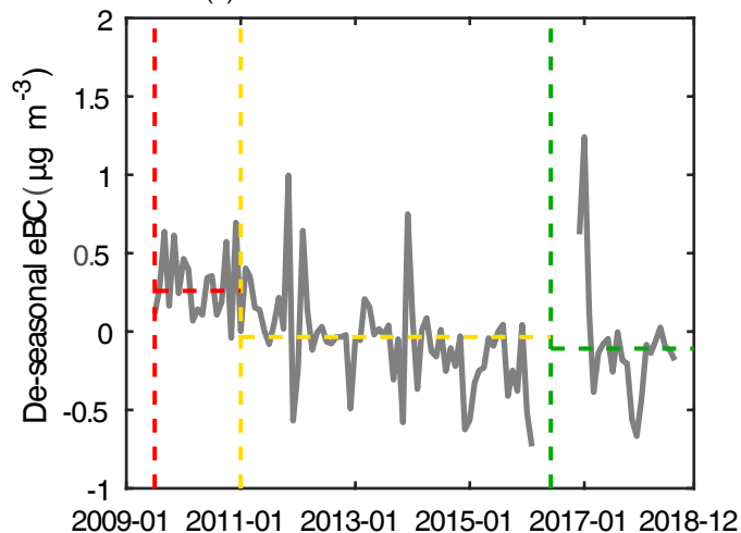
(c) eBC mass concentration at LTR
