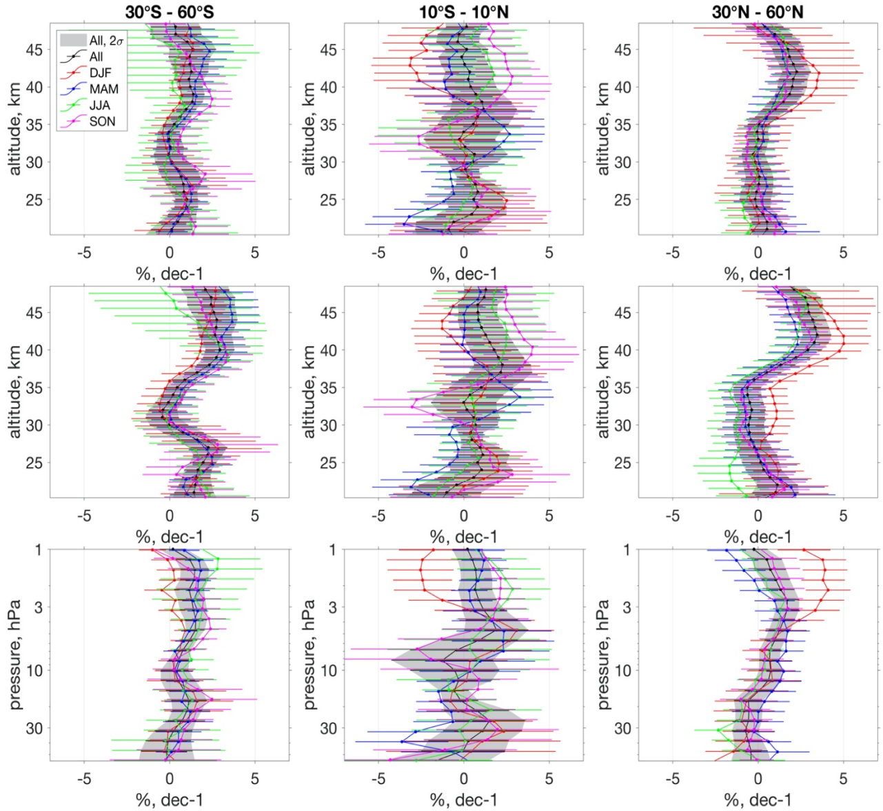
Figure S5. Vertical profiles of seasonal (red, blue, green, magenta) and yearly (black) ozone trends in 2000-2018 from CCI (top panels), SOO (middle panels) and GOZCARDS (bottom panels). The results are shown for three selected latitude bands. Error bars and shaded area (gray) are 2-sigma uncertainties.
