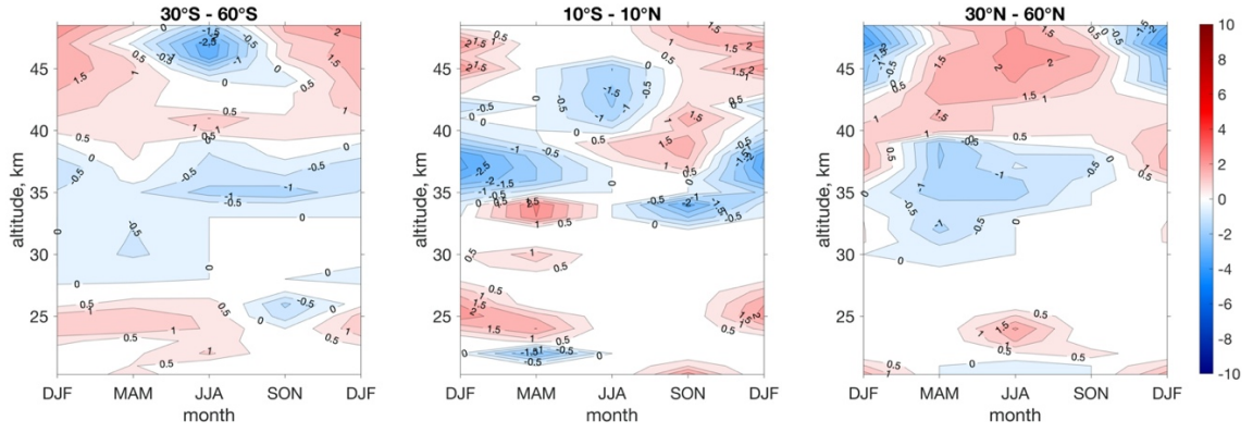
Figure S4. Altitude-seasons variation of the difference of the seasonal trends (mean[CCI, SOO] minus mean[GOZCARDS, SWOOSH]), calculated over 2000-2018 for three selected latitudinal bands.
