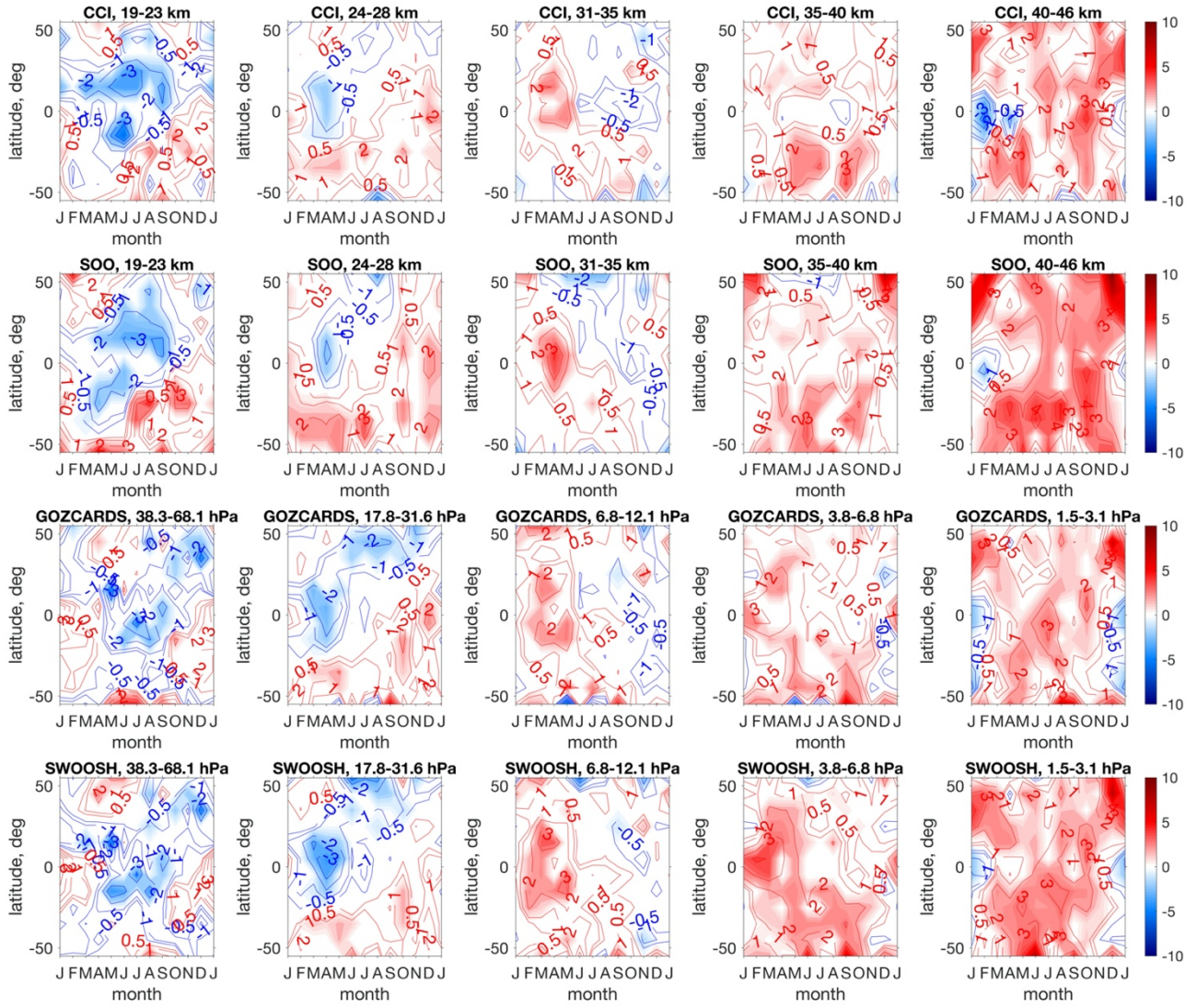
Figure S2. Latitude-months variation of linear trends in ozone for each of the merged data sets calculated over 2000-2018 for five selected altitude/pressure bands. The shading denotes trends that are significant at the 95% level.
