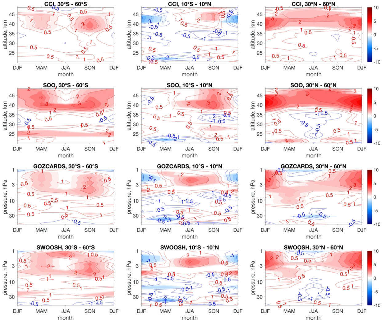
Figure S1. Altitude-seasons variation of linear trends in ozone for each of the merged data sets calculated over 2000-2018 for three selected latitudinal bands using method #2 (see description in the Manuscript). Data are presented on their natural vertical coordinate: altitude grid for CCI and SOO and pressure grid for GOZCARDS and SWOOSH. The shading denotes trends that are significant at the 95% level.
