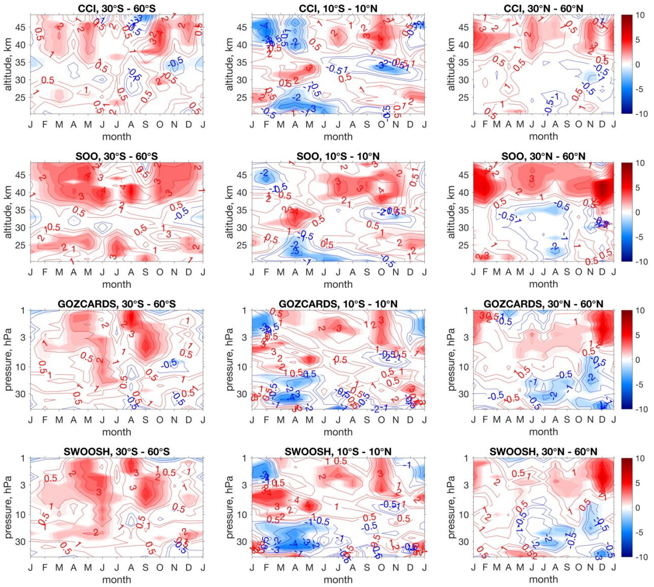
Figure S3. Altitude-months variation of linear trends in ozone for each of the merged data sets calculated over 2000-2016 for three selected latitudinal bands. Data are presented on their natural vertical coordinate: altitude grid for CCI and SOO and pressure grid for GOZCARDS and SWOOSH. The shading denotes trends that are significant at the 95% level.
