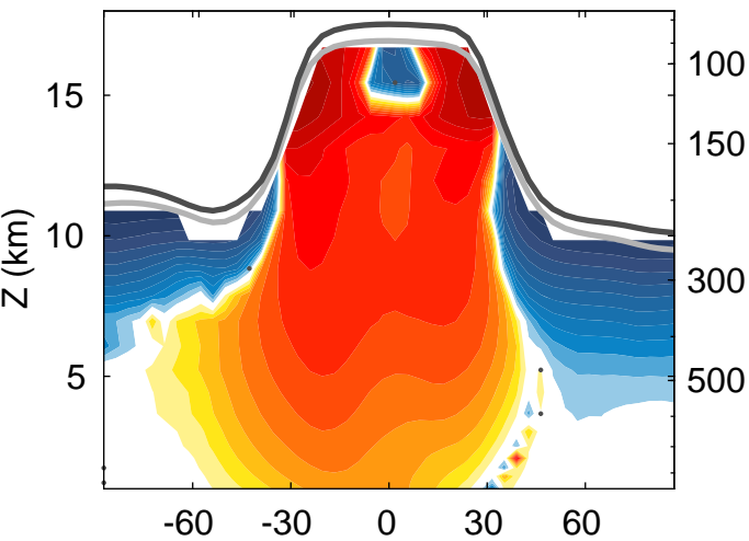
(a) st80 trends CMAM fODS
