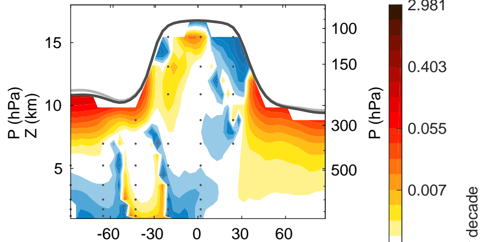
(b) st80 trends CMAM fGHG
