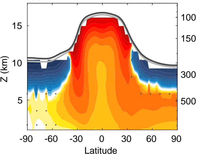
(c) st80 trends WACCM fODS
