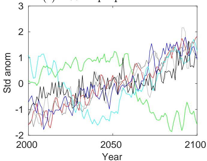
(c) st80 tropospheric column
