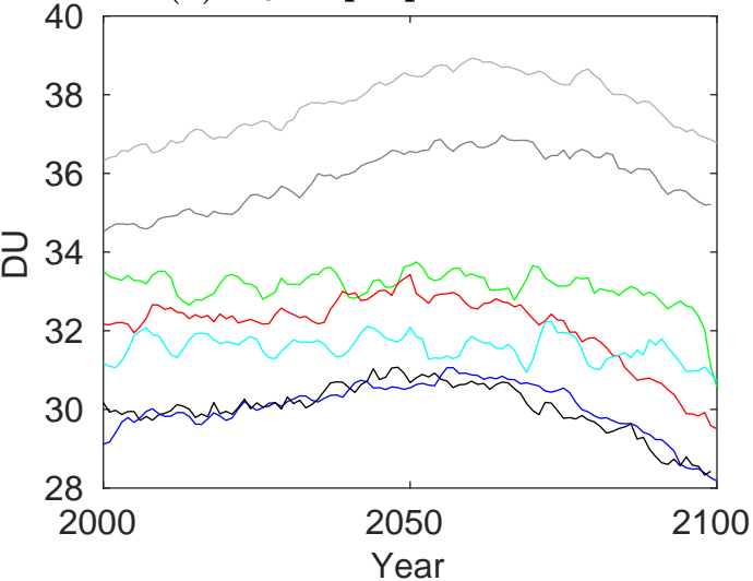
(c) st80 tropospheric column
