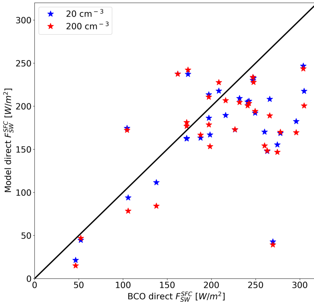
Figure S1. Comparison between the surface short wave flux ( F_{SW}^{SFC} ) observations at the Barbados Cloud Observatory (BCO; x-axis) and the model results (y-axis) for the NARVAL2 month (August 2016). For NARVAL1 no radiation measurements at the surface at BCO are available. Blue stars represent clean conditions ( CDNC = 20 \text{ cm}^{-3} ) while red stars polluted conditions ( CDNC = 200 \text{ cm}^{-3} ). In this case the model results were co-located with the BCO to within 0.01^\circ . Black line mark the 1:1 line.
