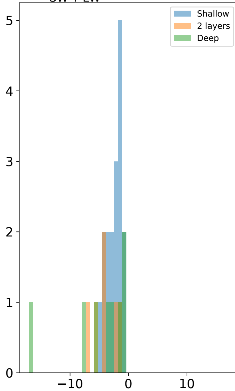
(b) \delta F_{SW+LW}^{TOA} [ W m^{-2} ] NARVAL 1
