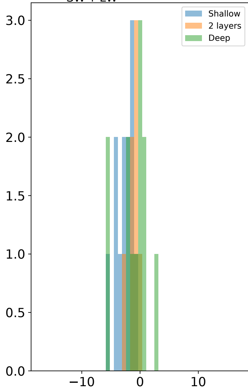
(c) \delta F_{SW+LW}^{TOA} [ W m^{-2} ] NARVAL 2
