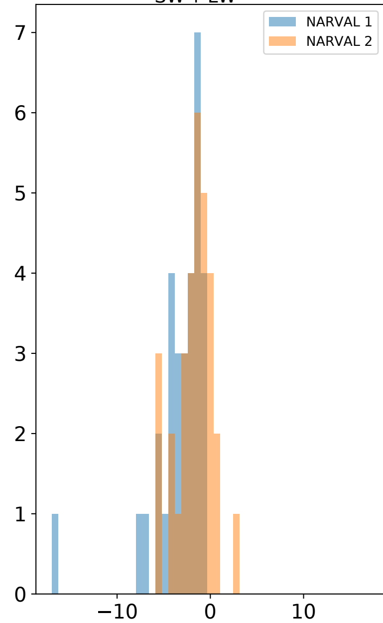
(a) \delta F_{SW+LW}^{TOA} [ W m^{-2} ]
