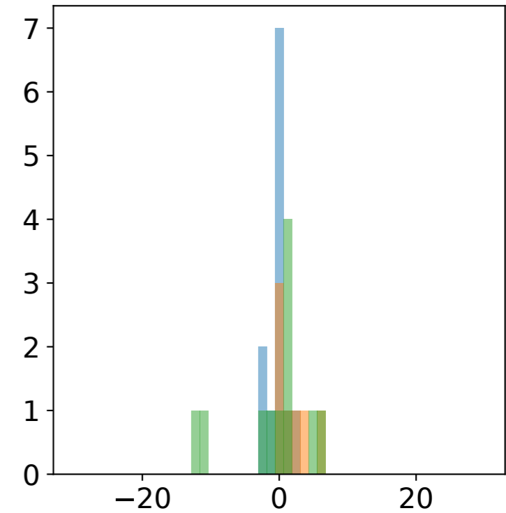
(h) \delta Q_R [ \text{W m}^{-2} ]
