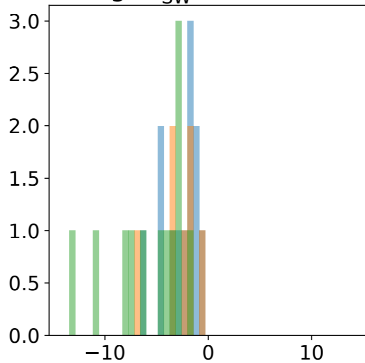
(g) F_{SW}^{TOA} [ \text{W m}^{-2} ]
