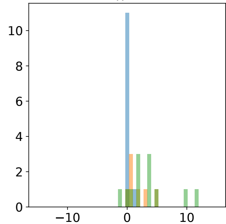
(h) \delta Q_R [ \text{W m}^{-2} ]
