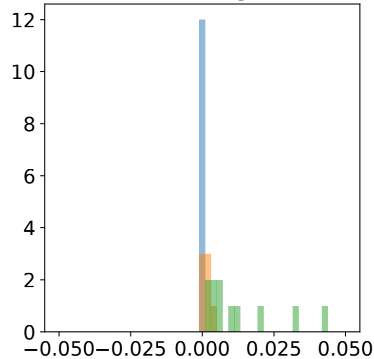
(g) F_{SW}^{TOA} [ \text{W m}^{-2} ]
