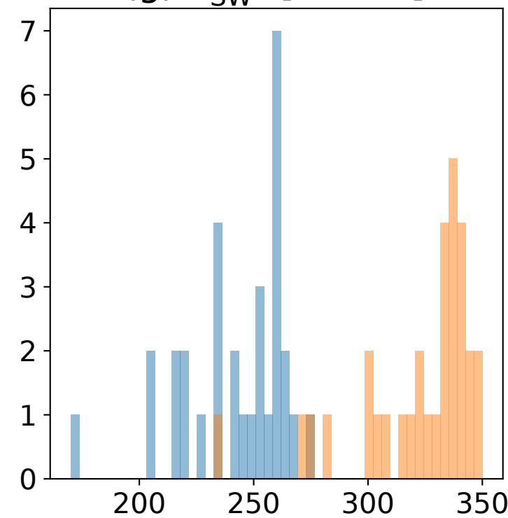
(g) F_{\text{SW}}^{\text{TOA}} [ \text{W m}^{-2} ]
