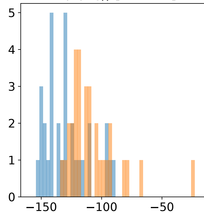
(h) Q_{\text{R}} [ \text{W m}^{-2} ]
