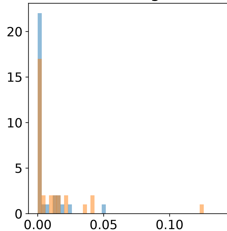
(g) F_{\text{SW}}^{\text{TOA}} [ \text{W m}^{-2} ]
