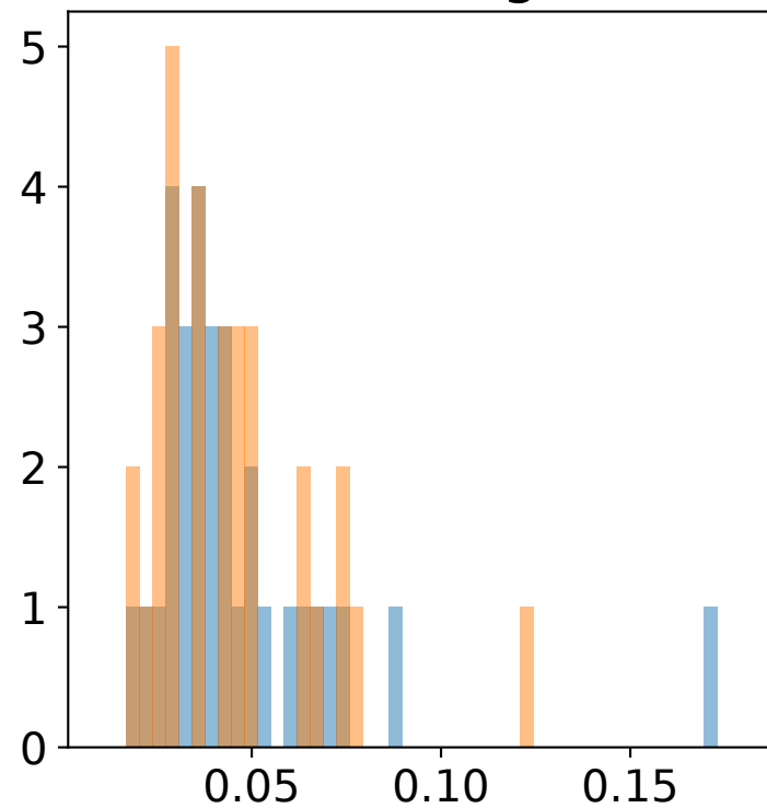
(f) F_{\text{LW}}^{\text{TOA}} [ \text{W m}^{-2} ]
