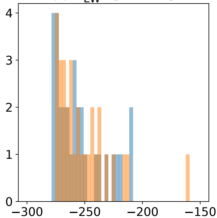
(f) F_{\text{LW}}^{\text{TOA}} [ \text{W m}^{-2} ]
