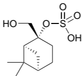
\beta -pinene-OS-2 c
