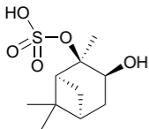
\alpha -pinene-OS-2 a
