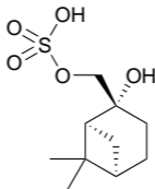
\beta -pinene-OS-1 c
