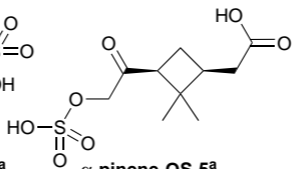
\alpha -pinene-OS-5 a
