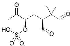
\alpha -pinene-OS-4 b
