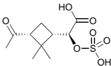
\alpha -pinene-OS-6 a
