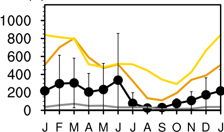
(a) Banizoum 13.5° N, 2.7° E
