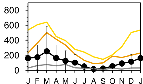
(b) Cinzana 13.3° N, -5.9° E
