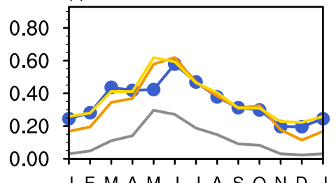
(f) Dakar 14.4° N, -17.0° E
