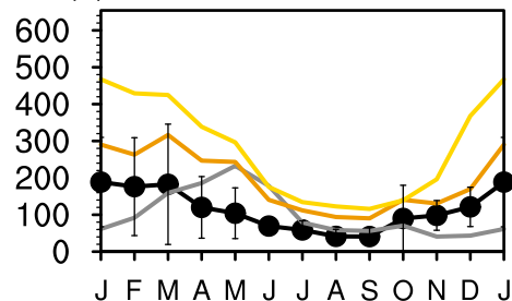
(c) M'Bour 14.4° N, -17.0° E
