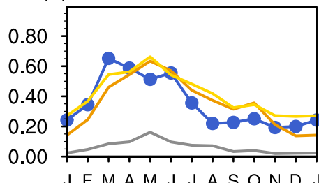
(e) IER_Cinz 13.3° N, -5.9° E
