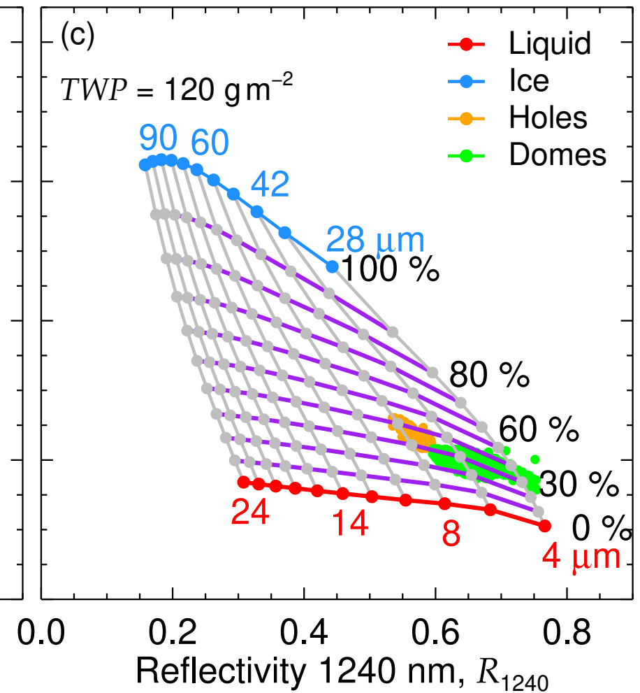
Homogeneous: constant TWP
