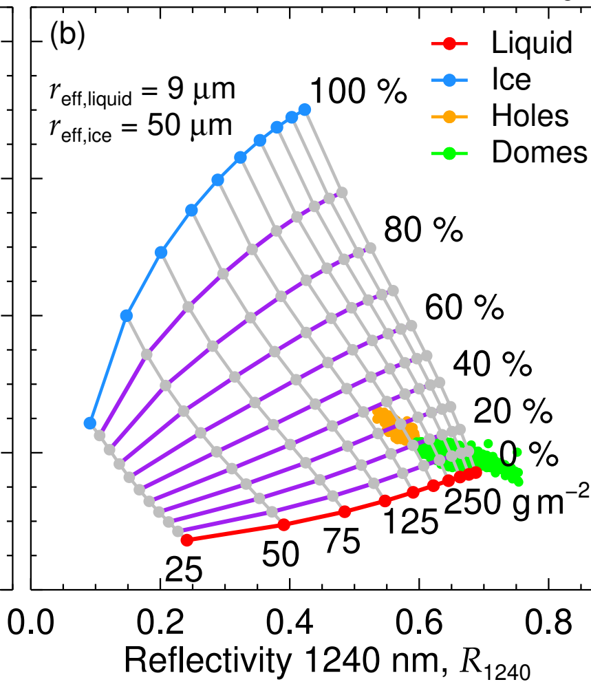
Homogeneous: constant r_{\text{eff}}
