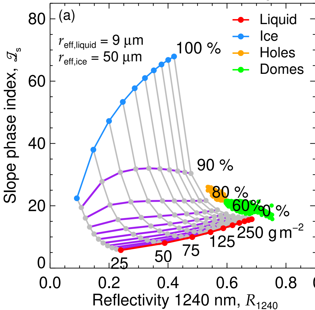
Two layers: constant r_{\text{eff}}
