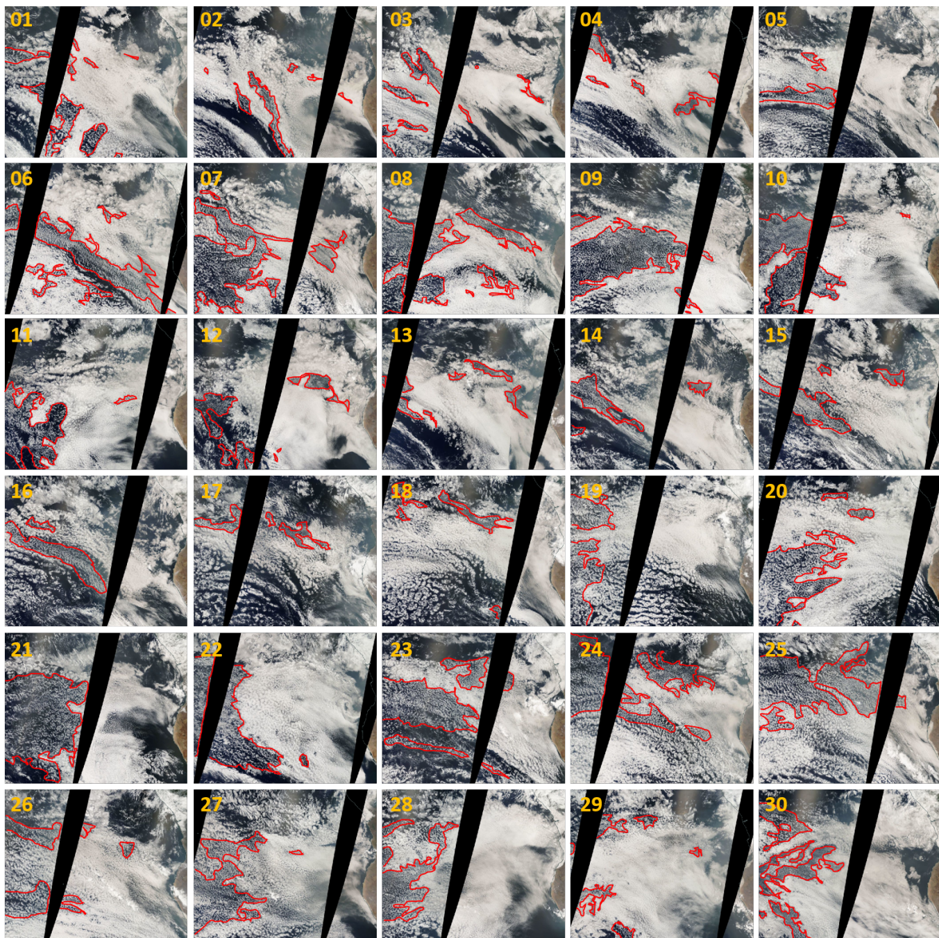
Figure S 1. Examples of the manual identification of open cell regions (outlined in red) from day-time MODIS Terra imagery, covering the period from the 1st to 30th September 2010. The MODIS imagery was obtained from NASA Worldview.
