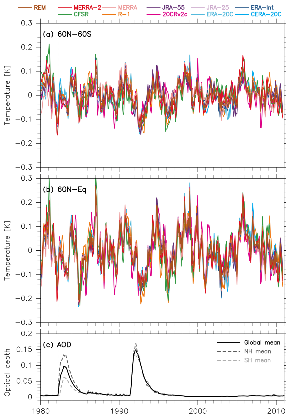
Figure 1. (a) Time series of the temperature residual R(t) (including volcanic signals and random variations) averaged for (a) 60^{\circ}\text{N} – 60^{\circ}\text{S} and (b) 60^{\circ}\text{N} –Equator as obtained from the 1980–2010 MLR analysis for 10 reanalysis data sets as well as the reanalysis ensemble mean (REM) (see legend at top). Three-month running means have been applied to each time series. (c) Time series of aerosol optical depth at 550 nm in the stratosphere (Sato et al., 1993; obtained from https://data.giss.nasa.gov/modelforce/strataer/ (last access: 25 July 2018); black solid for the global mean, dashed darker grey for the NH mean, and dashed lighter grey for the SH mean). For all panels, vertical dashed lines indicate the start dates of the two volcanic eruptions.
