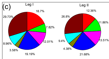
Mean fraction of aerosol types
