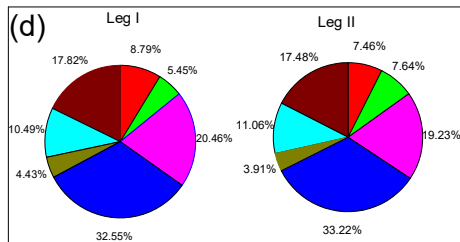
Mean fraction of MSA subtypes
