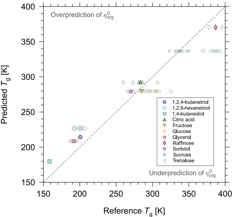
(a) T_g estimation method from DeRieux et al. (2018)
