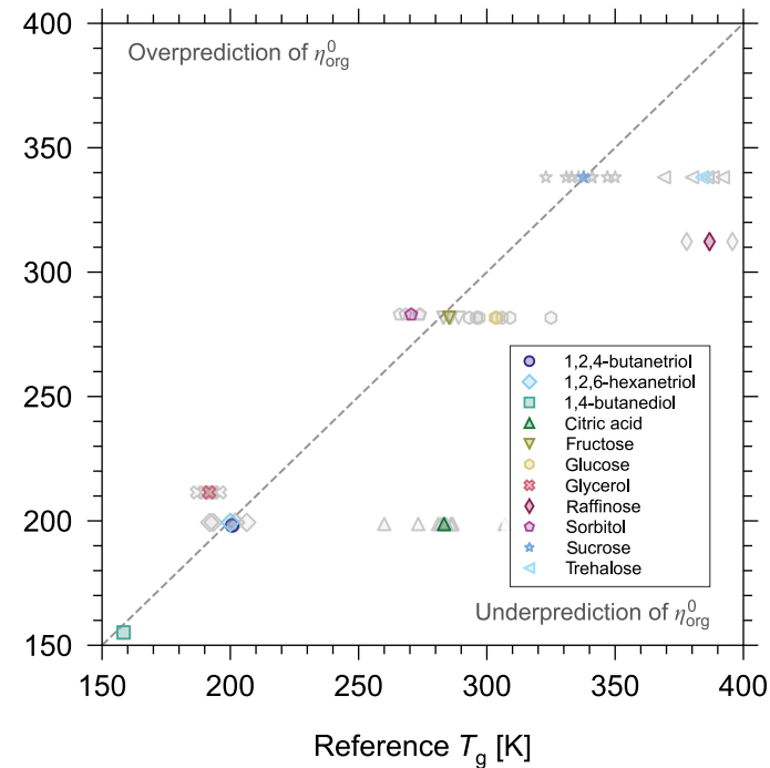
(b) T_g estimation method from Shiraiwa et al. (2017)
